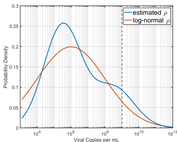
Figure 2: Probability density functions for \rho . The estimated distribution used in this work is shown along with a log-normal distribution centered at 10^6 /\text{mL} . The vertical line at 10^9 /\text{mL} indicates our “nominal \rho_0 ” of 1000 /\text{nL} . 10% of the estimated \rho distribution lies above this line and 7% of the log-normal distribution lies above it.
