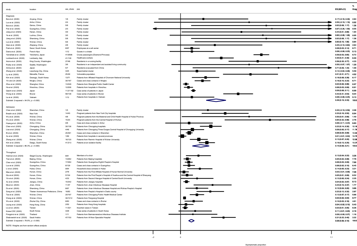
Figure 3. Forest plot of the proportion of asymptomatic cases. ES is the estimated asymptomatic proportion, with 95% confidence intervals (CI). I-squared is the percentage of between-study heterogeneity that is attributable to variability in the true effect, rather than sampling variation.
