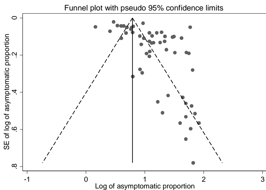
Figure S2b. Funnel plot of the 57 studies on overall asymptomatic infection.
