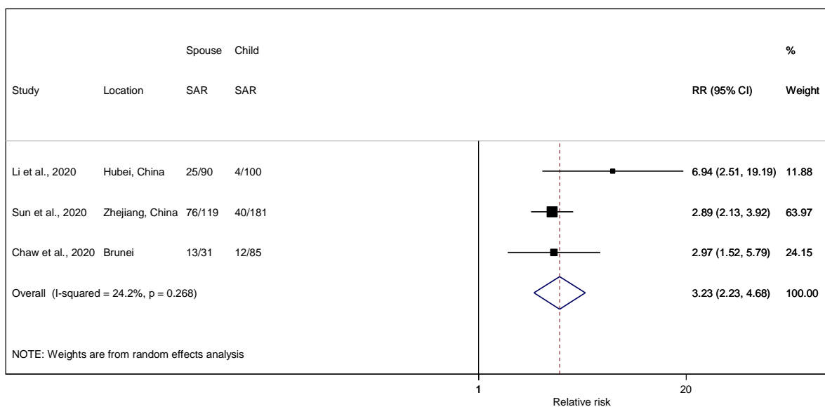
Figure S5. Forest plot of secondary attack rate in spouse and child of an index case. RR is the estimated relative risk ratio, with 95% confidence intervals (CI). I-squared is the percentage of between-study heterogeneity that is attributable to variability in the true effect, rather than sampling variation.
