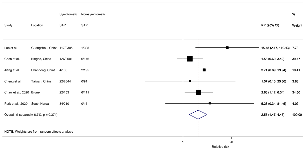
Figure S3. Forest plot of secondary attack rate by symptom status of index case. RR is the estimated relative risk ratio, with 95% confidence intervals (CI). I-squared is the percentage of between-study heterogeneity that is attributable to variability in the true effect, rather than sampling variation.
