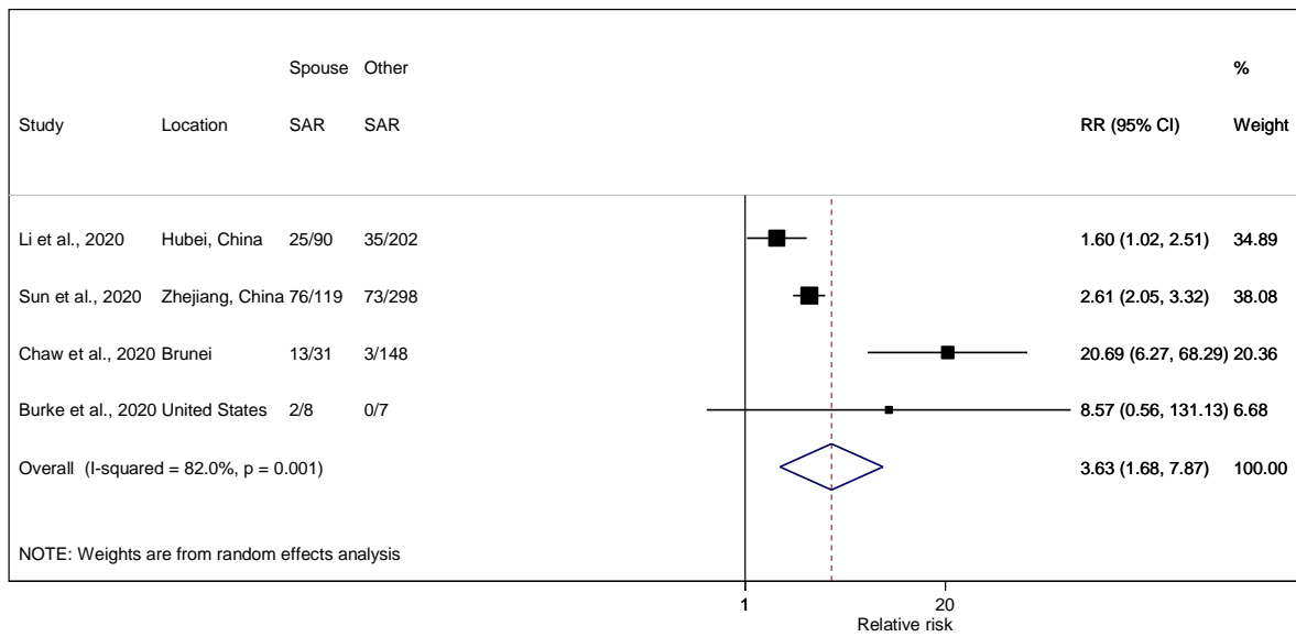
Figure S6. Forest plot of secondary attack rate in spouse and other household members (excluding child) of an index case. RR is the estimated relative risk ratio, with 95% confidence intervals (CI). I-squared is the percentage of between-study heterogeneity that is attributable to variability in the true effect, rather than sampling variation.
