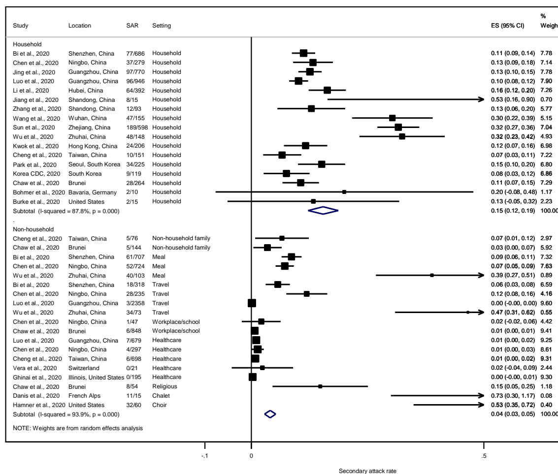
Figure 1. Forest plot of secondary attack rates (SAR) in different settings. ES is the estimated SAR, with 95% confidence intervals (CI). I-squared is the percentage of between-study heterogeneity that is attributable to variability in the true effect, rather than sampling variation.
