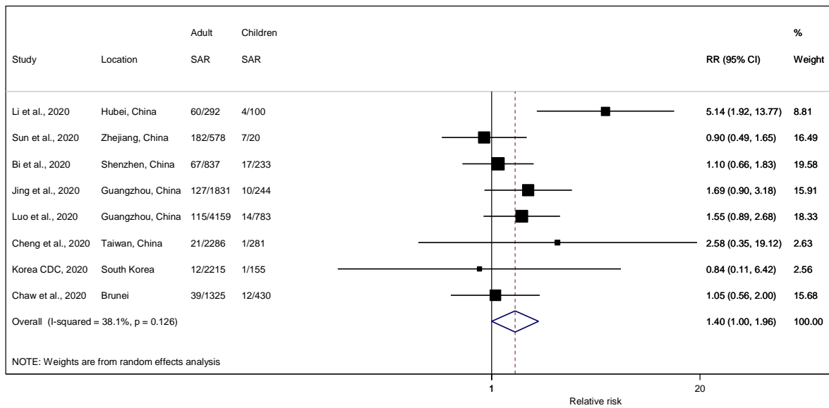
Figure S4. Forest plot of secondary attack rate in adults and children. RR is the estimated relative risk ratio, with 95% confidence intervals (CI). I-squared is the percentage of between-study heterogeneity that is attributable to variability in the true effect, rather than sampling variation.
