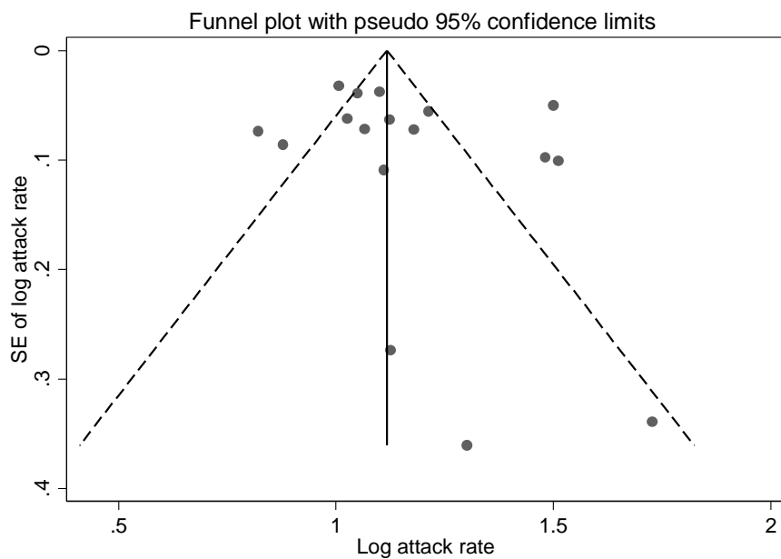
Figure S2a. Funnel plot of the 17 studies on household secondary attack rate.
