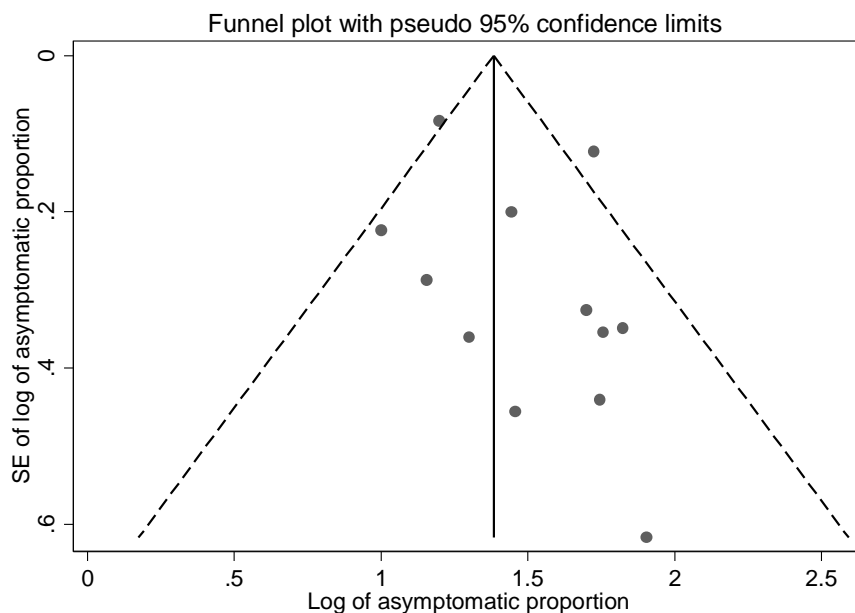
Figure S2c. Funnel plot of the 12 studies on asymptomatic infection in children.
