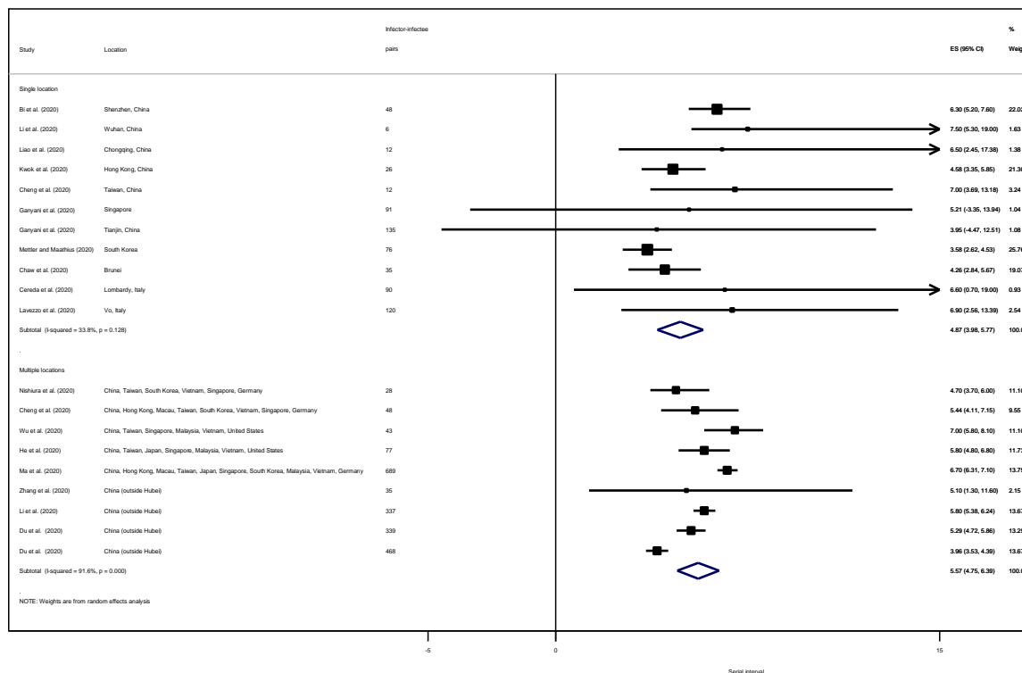
Figure 2. Forest plot of the serial interval (SI). ES is the estimated mean SI, with 95% confidence intervals (CI). I-
