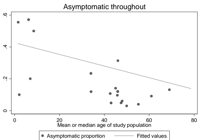
Figure S7. Scatter plots of asymptomatic infection and mean or median age of the study population
