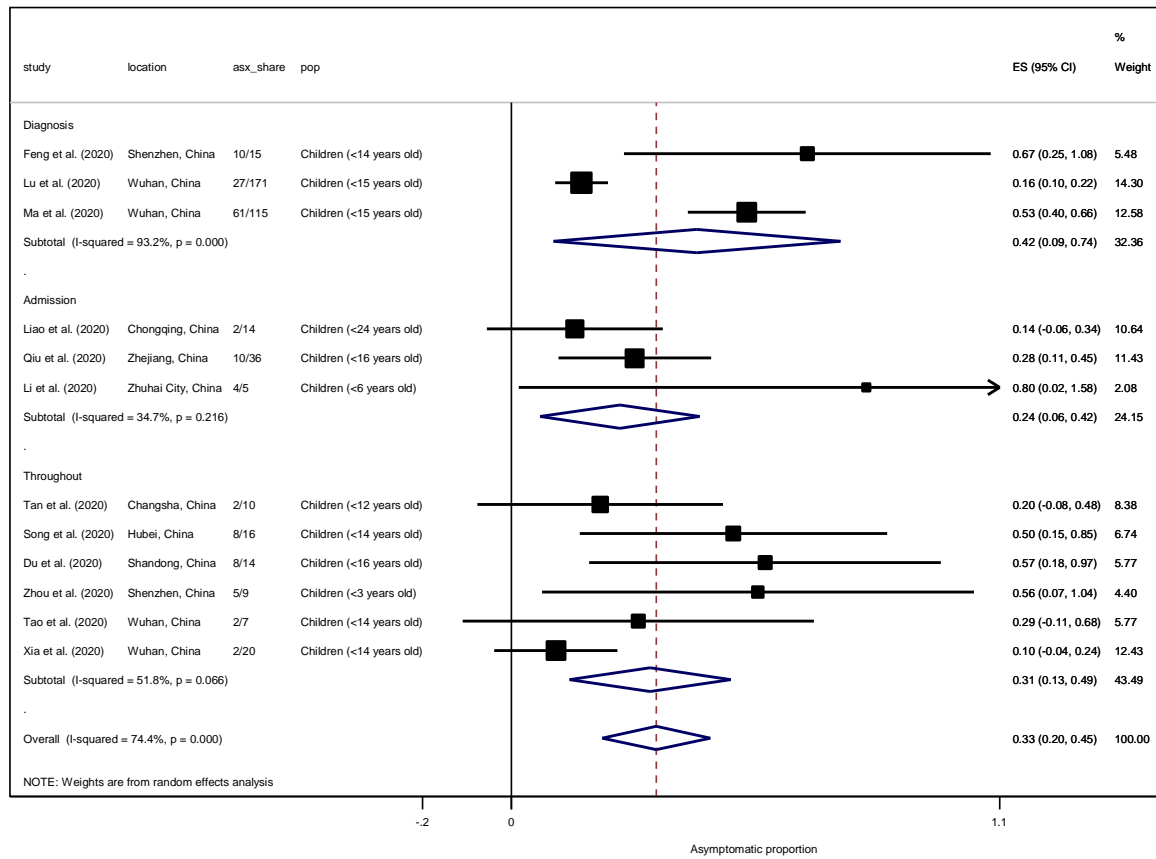
Figure S8. Forest plot of the proportion of asymptomatic cases in children at diagnosis, admission, and throughout the follow-up period. ES is the estimated asymptomatic proportion, with 95% confidence intervals (CI). I-squared is the percentage of between-study heterogeneity that is attributable to variability in the true effect, rather than sampling variation.
