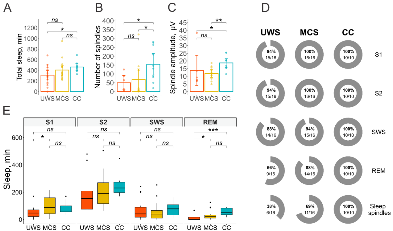
Figure 3 – Sleep stage distribution. (A) Total amount of sleep by group, (B) Number of sleep spindles by group. Only patients with present spindles (defined by visual screening) included (see Table 2), (C) Amplitude of sleep spindles by group. Only patients with present spindles (defined by visual screening) included (see Table 2), (D) The percentage of patients in each group, showing signs of the respective sleep stage during the 24h recording period. (E) Time spent in single sleep stages by group. UWS, unresponsive Wakefulness Syndrome; MCS, Minimally Conscious State; CC, Clinical Control; SWS, Slow-Wave Sleep; REM, Rapid Eye Movement Sleep; S1, S2, sleep stages 1 and 2, resp.; * p < .05 , ** p < .01 , *** p < .001 , ns not significant. Error bars are 95% confidence intervals.
