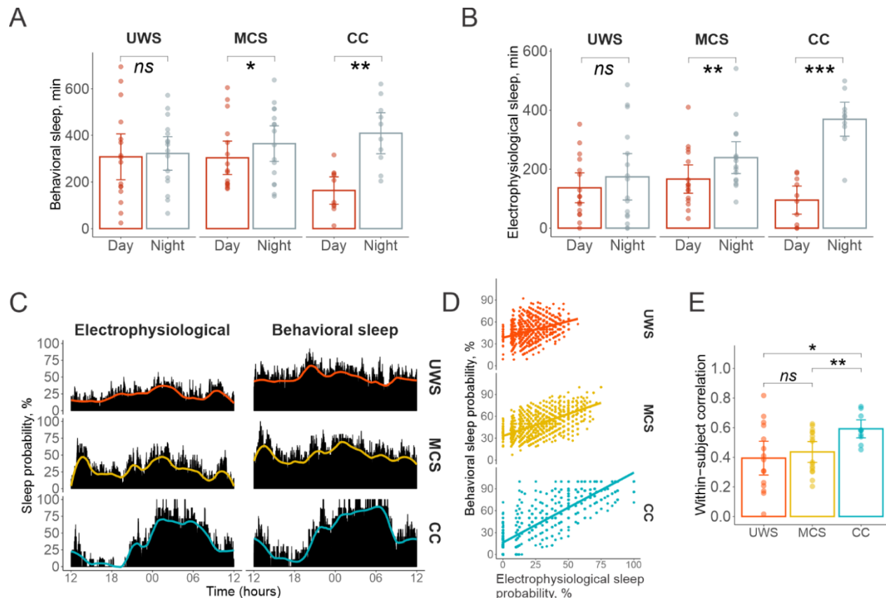
Figure 1 – Behavioral and electrophysiological sleep. UWS, Unresponsive Wakefulness Syndrome; MCS, Minimally Conscious State; CC, Clinical Control. (A) The amount of behavioral sleep (number of epochs with eyes closed) during the night and at daytime, for each group. (B) The amount of electrophysiological sleep evaluated by polysomnographic recording during the night and at daytime, for each group. (C) The distribution of sleep probability (percentage of patients who slept during the respective epoch) across all 2880 epochs. Solid lines show the results of smoothing according to the LOESS algorithm with the smoothing span of 0.2 by means of ggplot2 R package. (D) Scatterplots relating the probabilities (in %) that a particular epoch was a sleep epoch as scored with electrophysiological and behavioral measures (each dot represents one epoch). Note that the whole graph is “larger” for CC than for UWS and MCS, indicating a higher behavioral-electrophysiological correspondence among CC patients than DOC patients. There were epochs when all CC patients slept, and epochs when all of them were awake, but there were no such epochs in the two DOC groups. (E) Behavioral-electrophysiological sleep Kendall correlations calculated within each subject (dots) across epochs and averaged for each group (columns). * p < .05 , ** p < .01 , *** p < .001 , ns not significant. Error bars are 95% confidence intervals.
