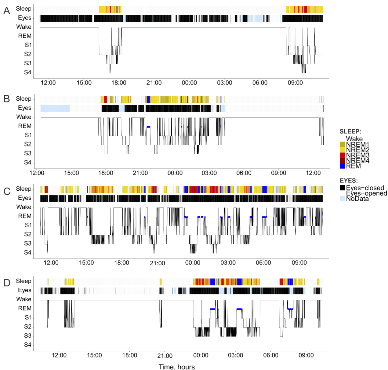
Figure 2 - Exemplary hypnograms of four patients. (A) an UWS patient who remained awake at night but slept during the day; (B) an MCS patient with close-to-normal sleep distribution; (C) an UWS patient with uniformly distributed sleep over the 24h period; (D) a CC patient with a pattern of well-structured sleep during the night and an afternoon nap. Notes: Sleep – electrophysiological sleep, Eyes – behavioral sleep.
