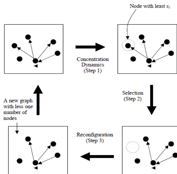
FIGURE 5: Schematic portrayal of the graph dynamics.
