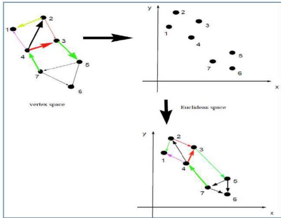
140 FIGURE 6: Schematic illustration transformation of the graph from vertex space to Euclidean space
