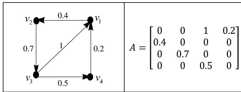
FIGURE 2: A fuzzy graph and its adjacency matrix.
