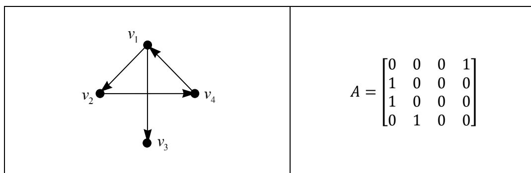
58 FIGURE 1: A directed graph with its adjacency matrix.
