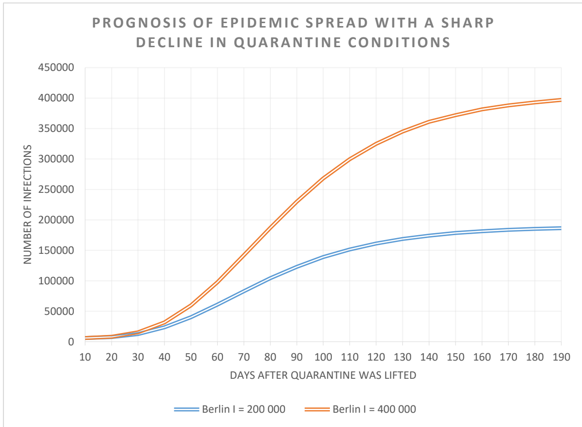
Fig. 2: Prognosis of epidemic spread with a sharp decline in quarantine conditions
