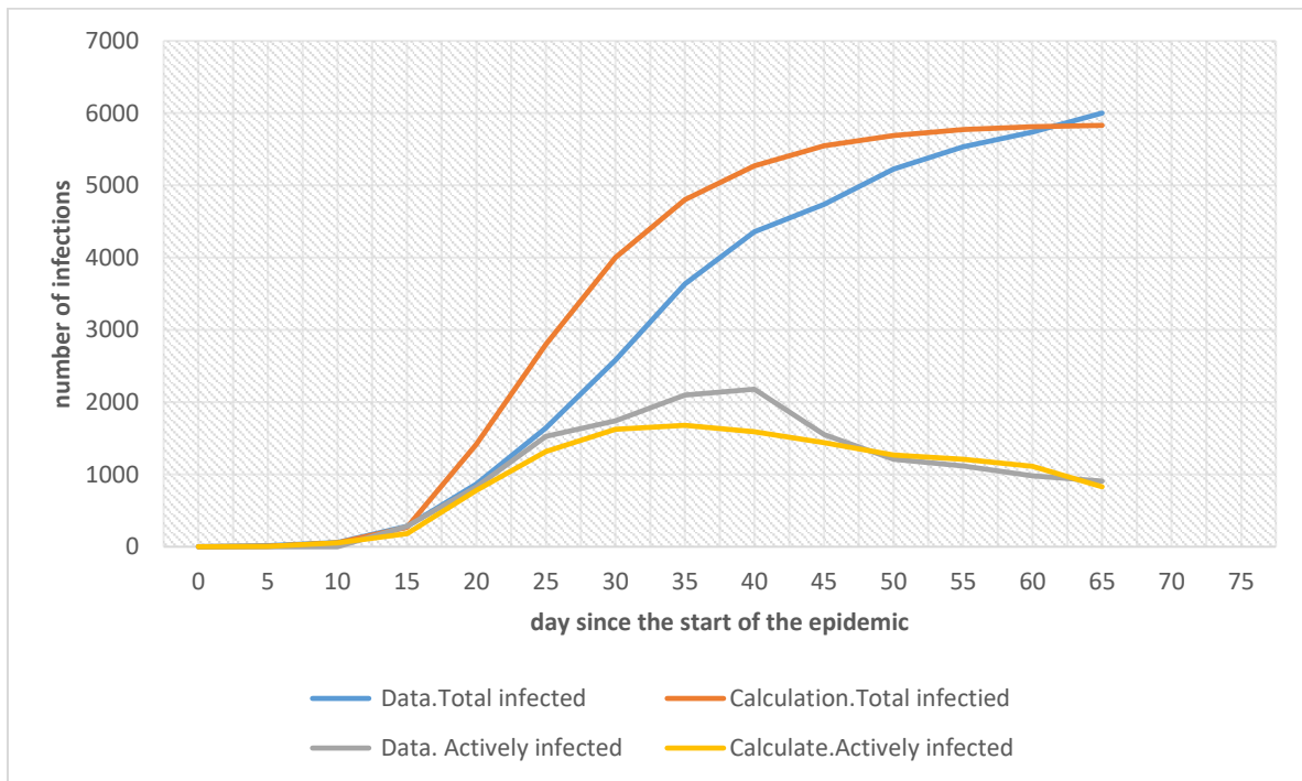
Fig. 3: The spread of the epidemic in quarantine conditions
