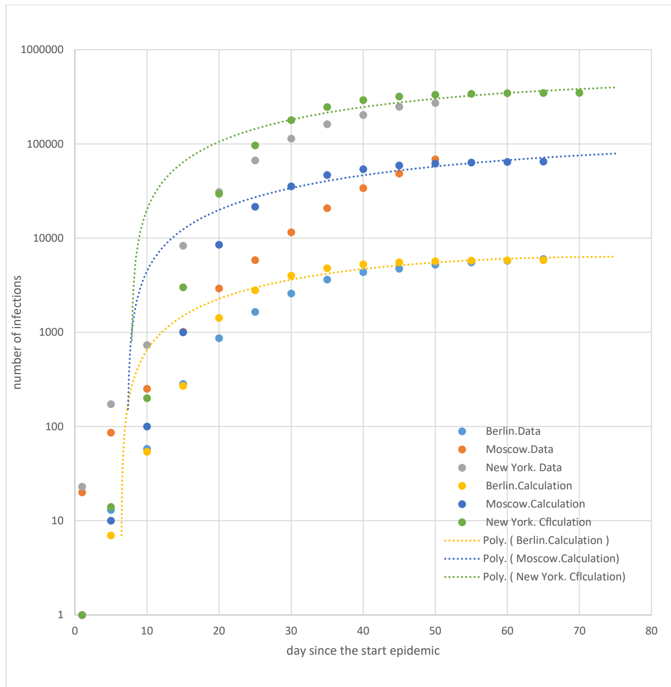
Fig. 1: The spread of the coronavirus epidemic cumulative infection
