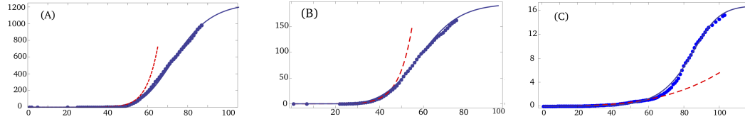
Figure 3: We plot the number (in thousands) of active cases C_n versus the number of days, n , in the alphabetical order for USA (A), Italy (B) and Japan (C). The red dashed-line is obtained by DG^2M , describes the first phase of the pandemic. The blue dashed-line comes from DG^2M , whereas DGRM result is shown as blue line. Together with the values of r and p obtained from DG^2M , (A) in case of the USA we have \alpha = 0.78 , and K = 1250,000 , (B) in case of Italy we have \alpha = 1.25 and K = 210000 . (c) In case of Japan, \alpha = 1.7 and K = 17000 .
