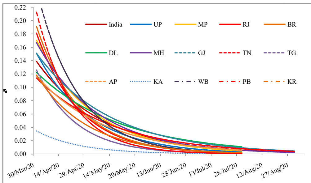
Figure 1: Trend of r_t for India and some states
