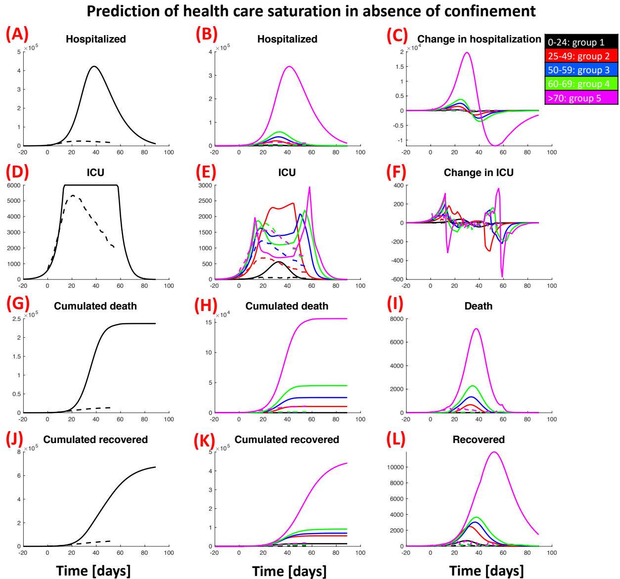
Figure S2: Prediction of pandemic spread and health care evolution in the absence of lockdown. Total number of hospitalized people (A), its age group distribution (B) and the daily variations (C); people in ICU (D), age group distribution in ICU (E) and the daily variations (F); cumulated deaths (G), age group distribution (H) and daily death (I); cumulative number of people recovered from hospitalization (J), age group distribution (K) and daily variations (L). Continuous lines show simulation results, dashed lines the actual data.
