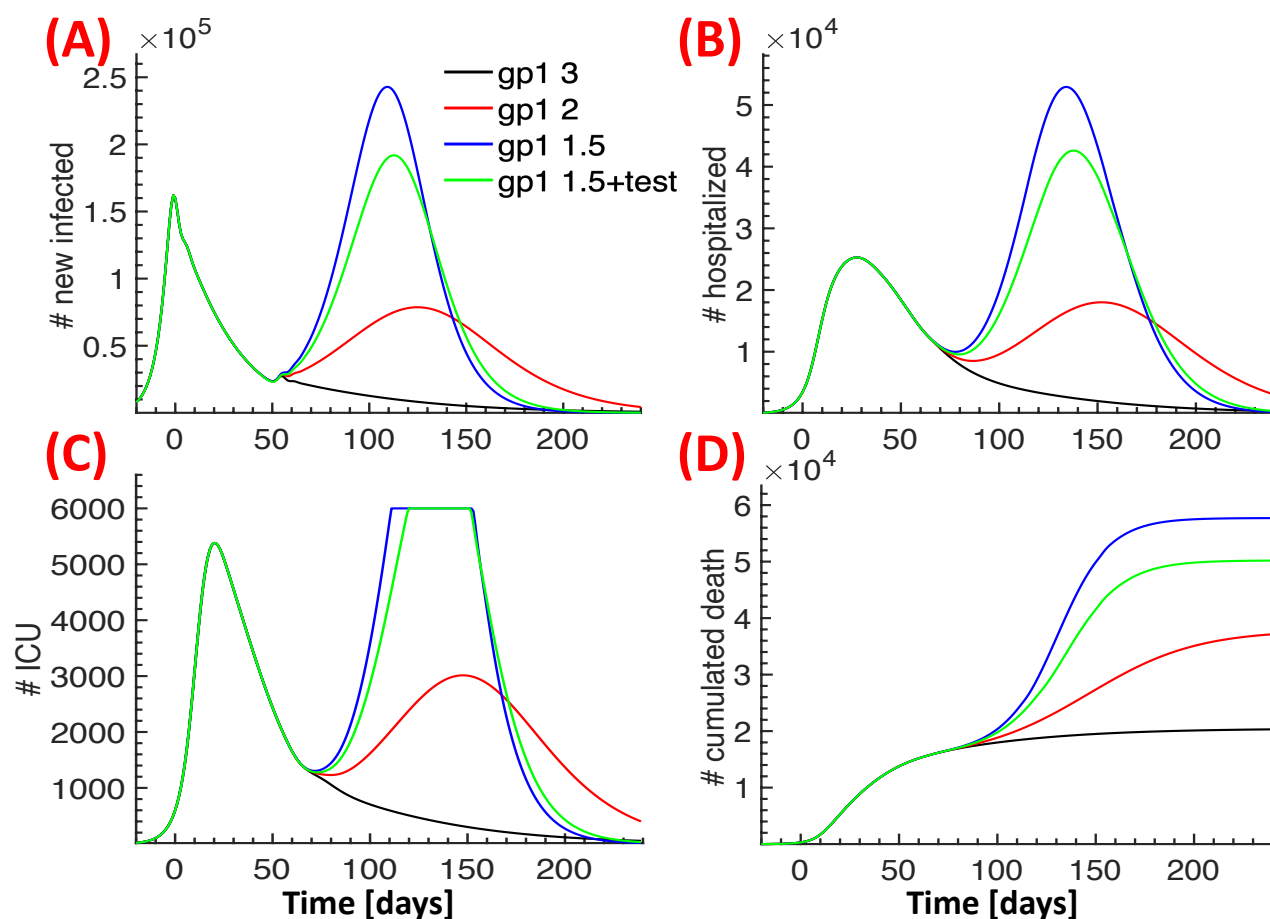
Figure 7: Possible effect of school openings after deconfinement. Comparison of four scenarios for the time after deconfinement where the infectiousness for group 2-4 is reduced by 3, whereas for group 1 it is reduced by a factor of 3 (black curves, corresponding to the red curves in Fig. 6), 2 (red curves) and 1.5 (blue curves). In the fourth scenario we added testing for group 1 (green curves). New daily infected (A), hospitalized (B), ICU occupancy (C), cumulative number of deaths (D).
