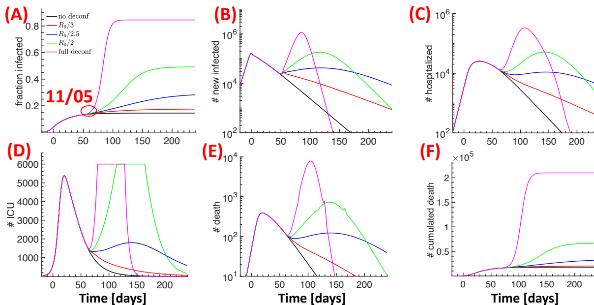
Figure 6: Effect of wearing masks after deconfinement. Wearing masks corresponds to a reduction in infectiousness and the reproduction number R_0 . Comparison of three scenarios where R_0 is reduced by 3 (strict mask wearing, red curves), 2.5 (less strict, blue curves) and 2 (insufficient, green curves). The results for no deconfinement (black curves) and full deconfinement with no restrictions (magenta curves) are also shown for comparison. Fraction of infected people (A), daily new infected (B), hospitalized people (C), ICU occupancy (D), daily deaths (E), and cumulative number of deceased (F).
