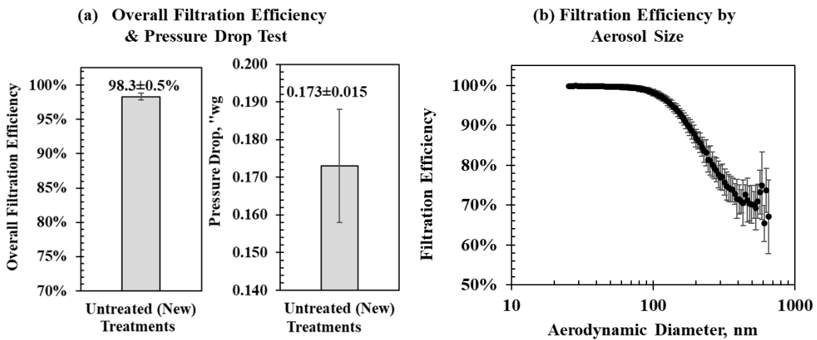
113 Figure 1. Test of an unqualified KN95 respirator: (a) overall filtration efficiency & pressure 114 drop test, and (b) filtration efficiency by aerosol size.
