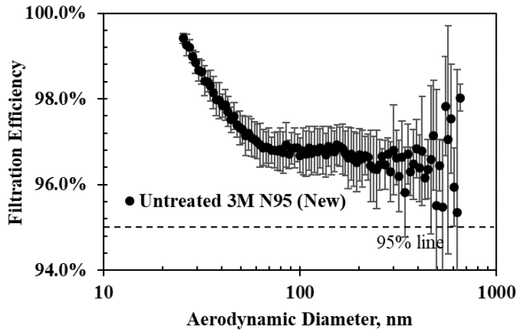
153 Figure 4. The most penetrating particle size (MPPS) for an untreated 3M N95 (new)
