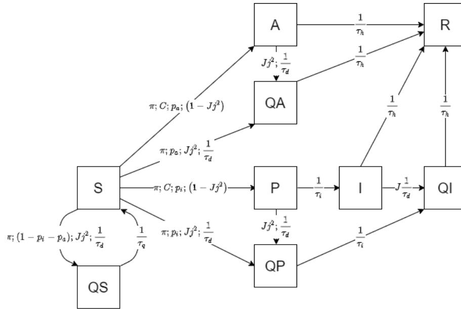
Figure 2: Model outline. Graphical representation of the interactions among the different compartments of the extended SIR model. S, susceptible; I, infected; R, recovered; A, asymptomatic; P, pre-symptomatic; QS, quarantined susceptible; QI, quarantined infected; QA, quarantined asymptomatic; QP, quarantined pre-symptomatic. Rates of transfer between compartments are a function of the parameters annotated on the arrows. A detailed description of such parameters is provided in "Materials and Methods" and Table 1.
