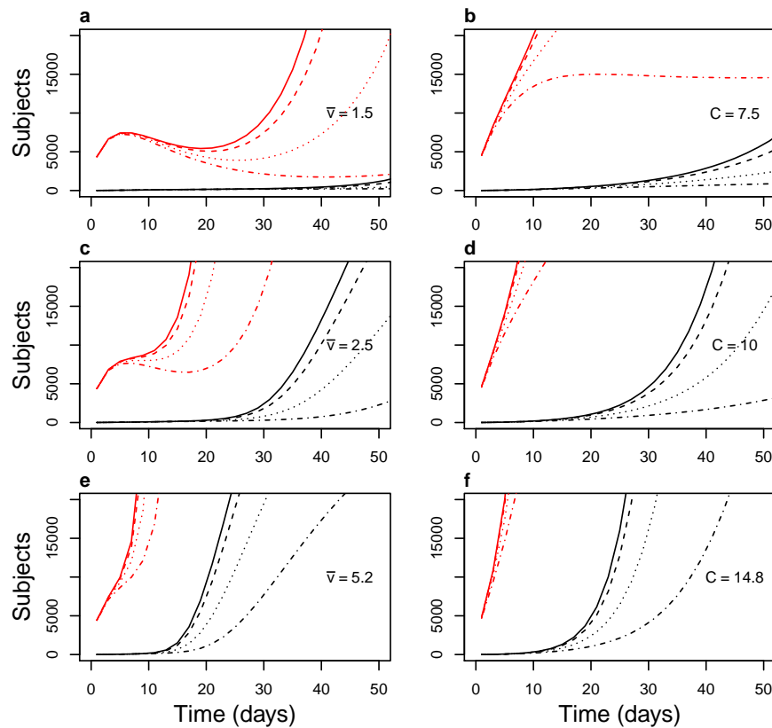
Figure 4: Detail of Figure 3 showing successful/unsuccessful suppression in the first 50 days. Suppression is achieved in the most optimistic scenario (contact rate 7.5, app users 75%) in the scenarios with fixed contact rate (right panels, upper), whereas its success varies from district to district in scenarios with density-dependent contact rate (left panels).
