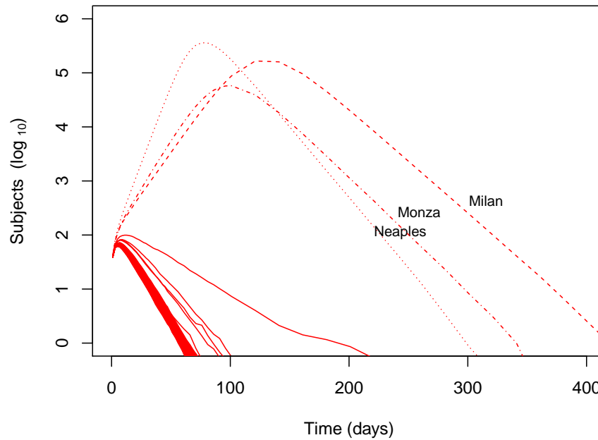
Figure 5: Epidemic curve for individual nodes (districts) in the scenario with average velocity \bar{v} = 1.5 and fraction of app users j = 25\% . The epidemic outbreak is entirely sustained by the three highest-density districts, whereas in the others the effective reproductive number is below 1.
