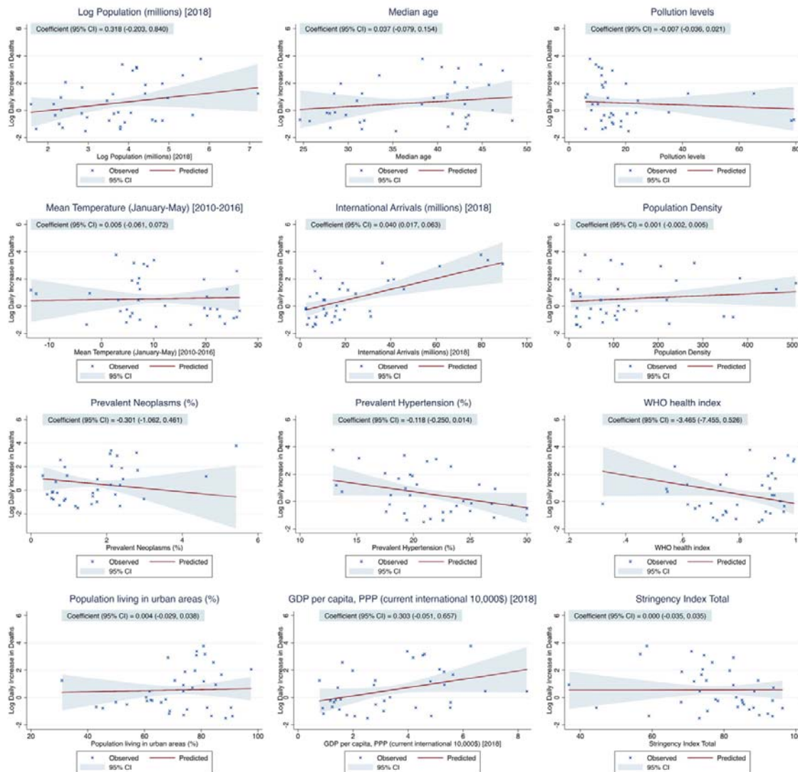
Figure 3. Predicted (based on the results of the multivariable linear regression) and observed country-level mortality rate (mean daily increase in deaths until the peak in mortality) as a function of each country-level predictor included in the multivariable model.
