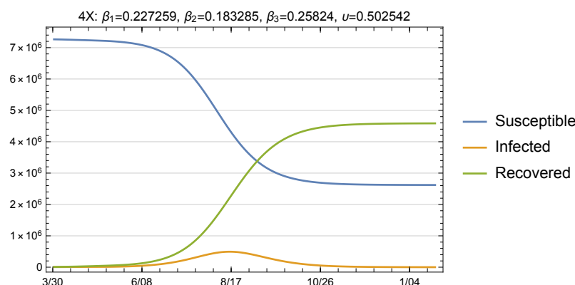
Fig 11. Susceptible, infected and recovered, 4X loading with fitted \beta and \nu
