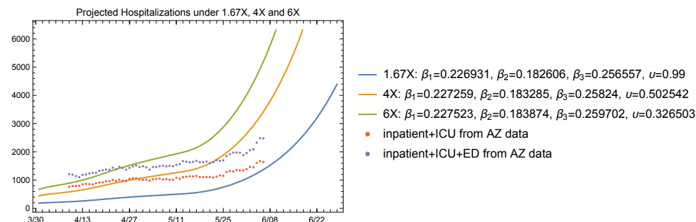
Fig 15. Hospitalized patients projected by the model with fitted \beta and v
