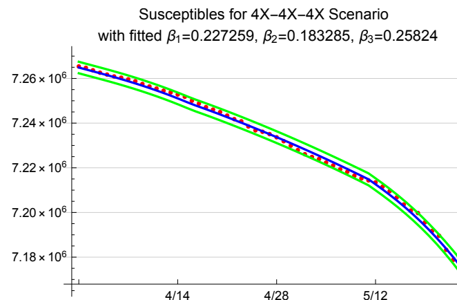
Fig 8. 95% prediction bands for susceptibles; red dots show presumed susceptibles under 4X scenario
