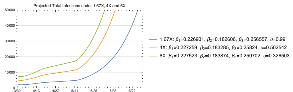
Fig 14. Total infected projected by the model with fitted \beta and v
