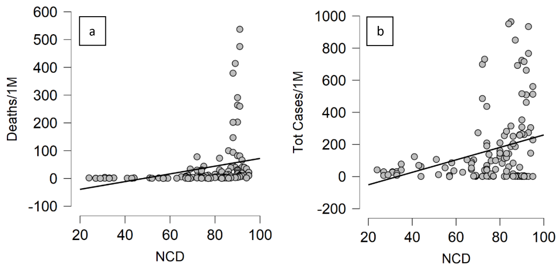
Figure 1. Graphical representation of correlations between noncommunicable chronic diseases death rate and COVID-19 mortality (a) and incidence (b) among countries.
