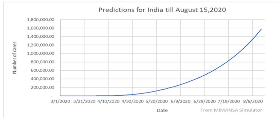
Fig. 4(b) : Predictions for India
