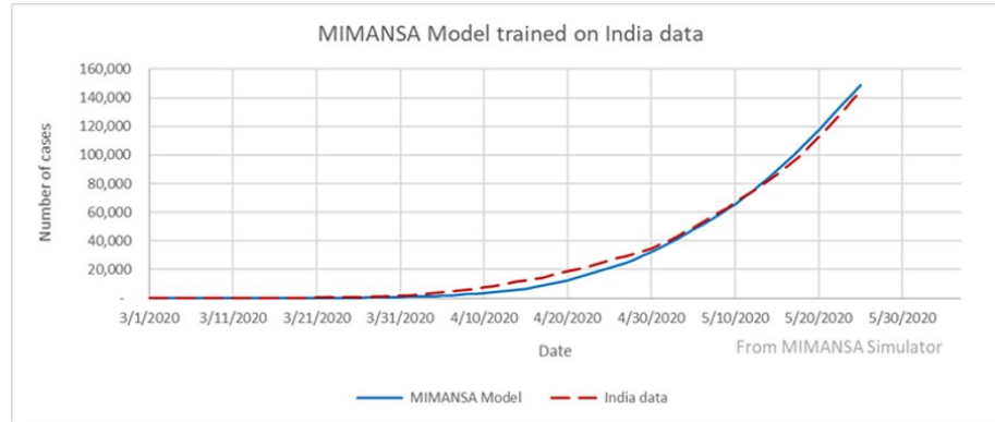
Fig. 4(a) : Trained model for India data
