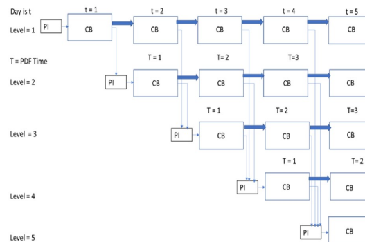
Figure 2b: Virus Proliferation Network Using the Computational Blocks, one for each day and level.
