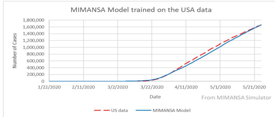
Fig. 5(a) Trained Model for USA data
