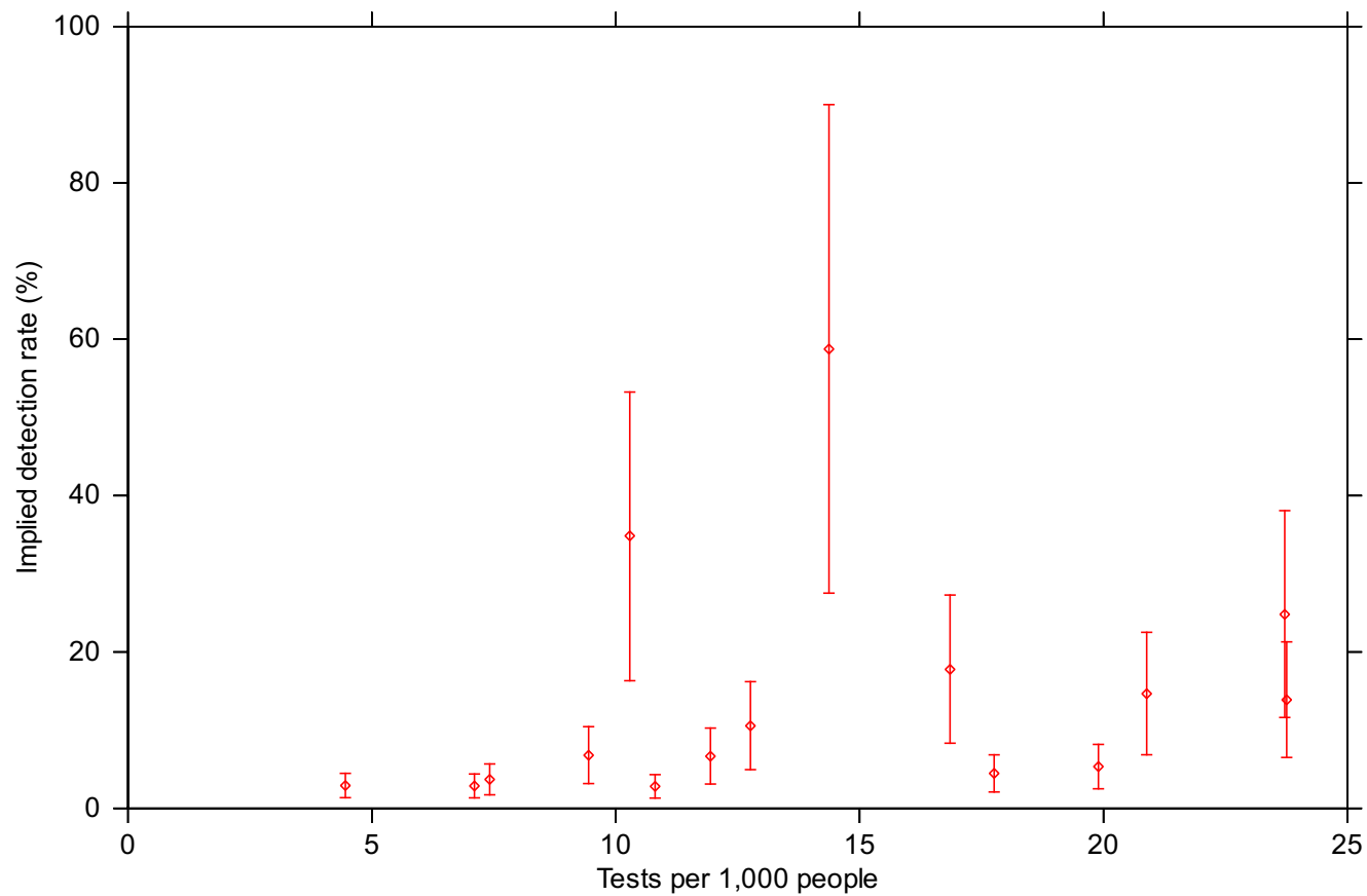
Figure 3. The implied true detection rate for each country versus the number of tests per 1,000 people: the median estimates (diamonds) and the 5–95% confidence intervals (vertical bars). All values are current as at 14 April 2020, except for Germany (testing data current as at 12 April 2020), Spain (testing data current as at 12 April 2020) and Sweden (testing data current as at 12 April 2020).
