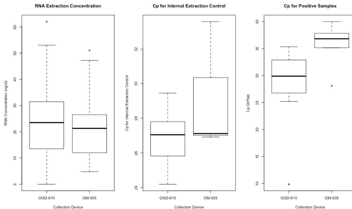
Supplementary Figure 1: (a) Comparison of RNA Extraction Yield where available for OGD-610 vs OM-505, (b) Comparison of Cp value for PrimerDesign Internal Extraction Control and (c) Comparison of Cp value for PrimerDesign Internal Extraction (for a subset of samples only), Control Cp and viral gene target Cpt and viral gene target Ct on OGD-610 and OM-505 on positive clinical samples from Diagnosis Cohort
