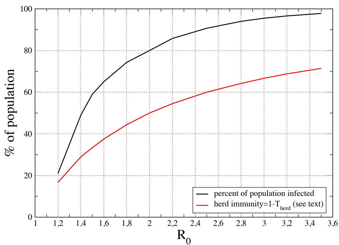
Percent of population contaminated and herd immunity as a function of R_0 .
