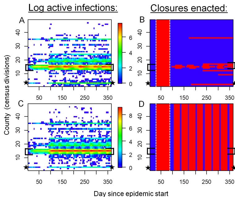
Figure 1: Spatiotemporal patterns of local COVID-19 cases and school/workplace closures. Panels show actual (confirmed plus not ascertained) number of COVID-19 cases (a,c) and time periods of workplace closure (red) and opening (blue) (b,d) in Ontario, Canada under local (a, b) and global (c, d) strategies. Disease dynamics are sporadic in low-population counties but endemic in high-population counties. The local strategy generates a similar disease burden to the global strategy but requires fewer person-days of closure. Optimal trigger prevalence is assumed (blue dashed lines, Fig. 2a-b). Brackets denote the Greater Toronto Area, star denotes Ottawa, and vertical dashed lines in (b, d) delineate the initial province-wide closure. All simulations were initialized with 250 exposed persons on day 1.
