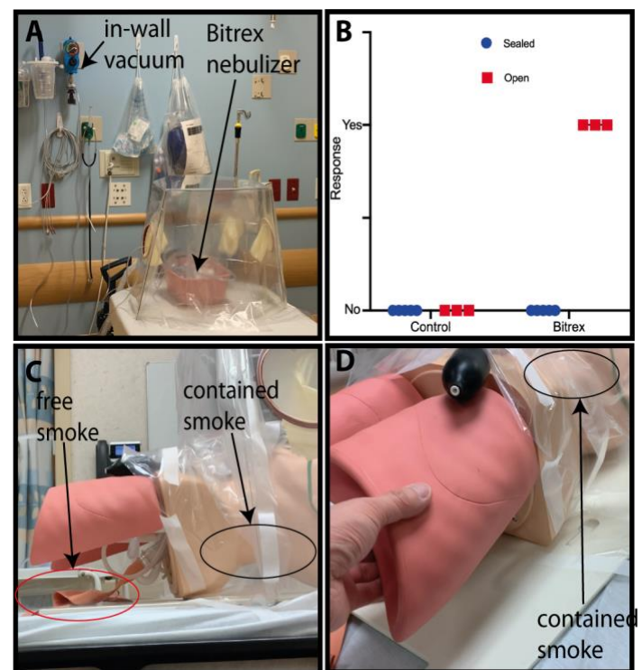
Figure 4: (A) Bitrex containment test setup with nebulized Bitrex or saline control inside the BADGER. Bitrex was delivered by oxygen nebulizer at 5 L/min. (B) Results of a double-blinded containment test. Zero out of 5 volunteers detected bitter taste when the BADGER was sealed, and suction applied at 100 mmHg to create outflow rate of 39 L/min. When the BADGER was unsealed and suction turned off, 3/3 in the Bitrex group and 0/3 in the saline group detected bitterness. (C) Smoke tests using ventilation smoke tubes (Grainger) while the mannequin was receiving 10 L/min of oxygen via facemask. Free smoke (red oval) was seen leaking from the bottom of the BADGER before vacuum suction was applied. (D) After suction was applied at 100 mmHg, coughs were simulated by compressing the mannequin's lungs; all the smoke was contained (black oval).
