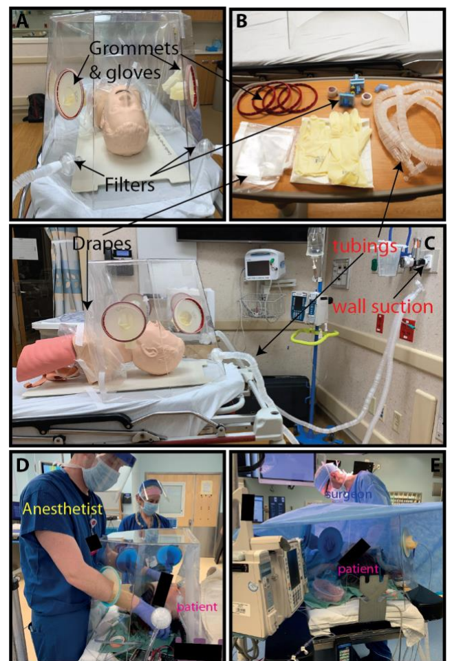
Figure 3: (A-C) Set up of the BADGER on a mannequin. The BADGER uses commonly available hospital supplies to create isolation and semi-sealed chamber. Accessories for each BADGER are: two viral HEPA filters, two 60 cm x 60 cm clear drapes, 5-10 m of 6 mm or 7 mm inner diameter tubing, one dual-limb breathing circuit tubing, 2 pairs of size 8.5 or 9 surgical gloves. Grommets and surgical gloves are assembled into sleeve-rings to seal the hand-ports. Drapes are taped to create overlapping opening for the torso/neck. (D-E) Clinical application of an earlier version of the BADGER on a patient for intubation (D) and intraoperative use (E).
