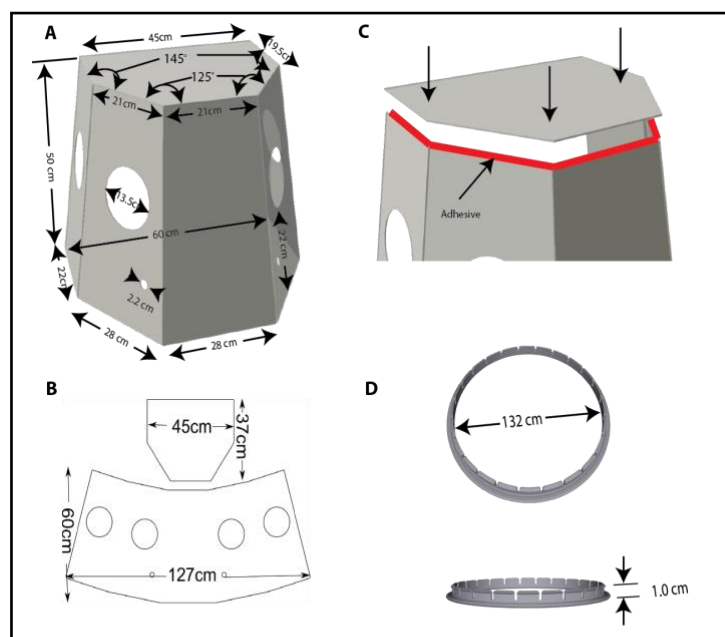
Figure 2: Configurations of the BADGER and grommet. (A) The BADGER has a tapered pentagonal shape with an overall height 50 cm and overall volume 95.8 L, four 135 mm diameter hand-ports and two 22 mm diameter outlets for filter placement. (B) The side panels can be constructed via bending or cutting into separate panels. (C) Top panel is glued to side panels using hot melt adhesive. (D) 3D-printed grommets, used to attach surgical gloves to the BADGER.
