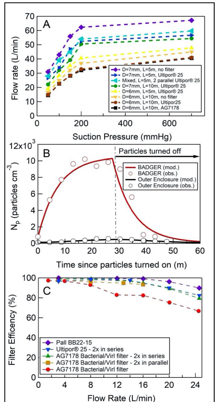
Figure 5: A) Air flow rates from a hospital room's in-wall vacuum suction source at various suction pressures, tubing inner diameters (D), tubing length (L), and viral filters (Ultipor25® or AG7178). Mixed setup: 2 Ultipor 25® filters connected in parallel to 1.8m of a dual-limb breathing circuit tubing (Adult UltraFlex® Dual-Limb breathing circuit) and 3.2 m of 7 mm inner diameter tubing. B) Particle containment result at outflow rate of 13 L/min. Sub-micrometer particle concentrations were measured in both the BADGER (red circles) and the exterior enclosure (black circles). For the well-sealed BADGER, greater than 90% of sub-micrometer particles generated in the BADGER were contained. C) Measured aerosol particle filtration efficiency for the selection of filter substrates and combination of filters used in this study. The filtration efficiency test was conducted using aerosol particles present in the room, where the mean particle diameter was 220 nm.
