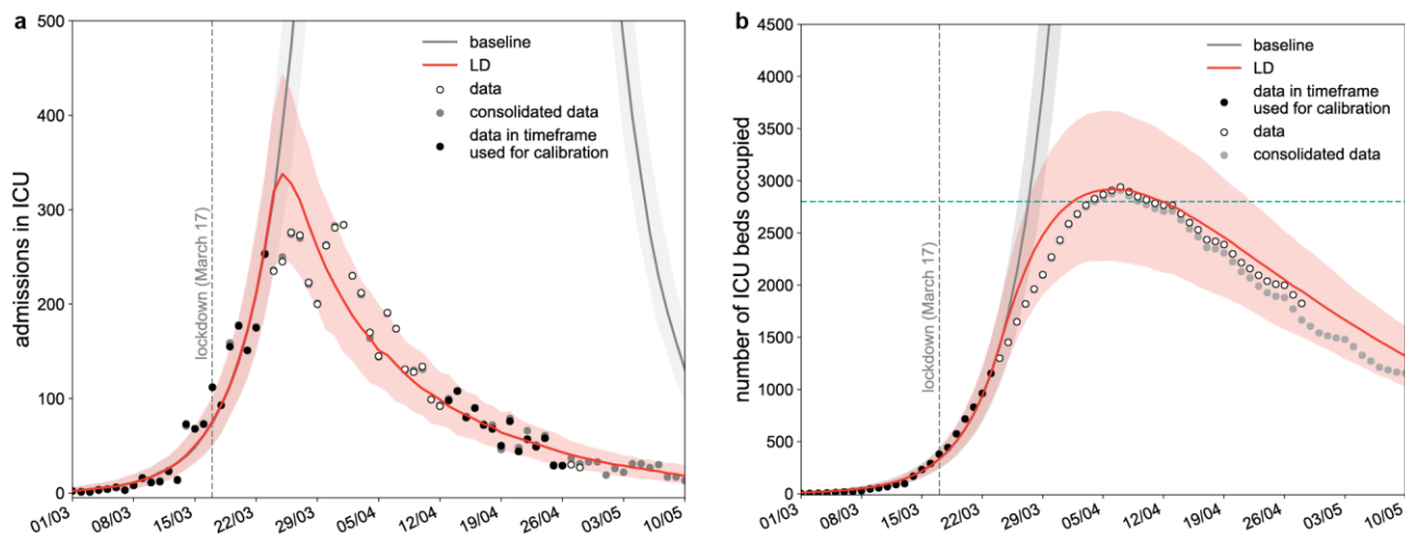
Figure 1. Simulated epidemic trajectories till May 11. (a) Simulated daily incidence of admissions in ICU over time. (b) Simulated number of ICU beds occupied over time. The fitted curve slightly overestimates the data, likely because it does not account for the transfer of patients in intensive care to less affected regions. Vertical dashed line refers to the start of the lockdown; curves and shaded areas correspond to median and 95% probability ranges, obtained from n = 500 independent stochastic runs; horizontal line refers to strengthened ICU capacity in the region to face the first COVID-19 wave; LD stands for lockdown. Black dots indicate data used for the calibration; grey dots indicate data that became available after the initial submission of this study.
