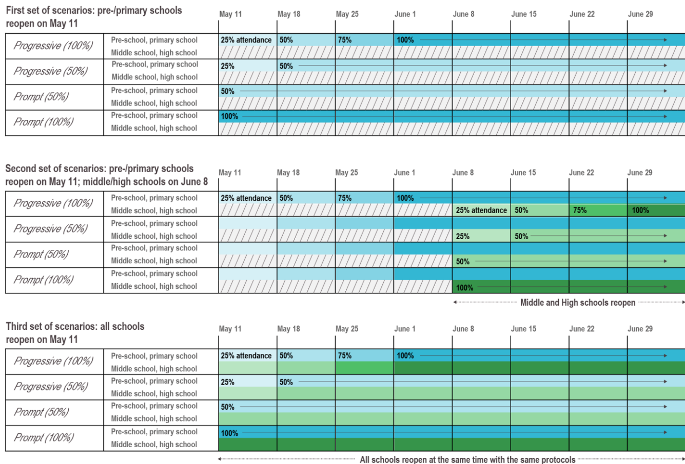
Figure 2. Protocols of school reopening. The first set of scenarios considers the reopening of pre-schools and primary schools only, on May 11, through Progressive (100%) , Progressive (50%) , Prompt (50%) , and Prompt (100%) protocols. Progressive (100%) : progressive reopening up to 100% attendance, where 25% of students go back to school on the 1 st week after lockdown is lifted, 50% on the 2 nd , 75% on the 3 rd , and 100% from the 4 th week till summer holidays. Progressive (50%) : progressive reopening up to 50% attendance, where 25% of students go back to school on the 1 st week after lockdown is lifted, and 50% from the 2 nd week till summer holidays. Prompt (50%) : partial reopening with 50% attendance from May 11. Prompt (100%) : full reopening with 100% attendance from May 11. Colors indicate school levels (blue for pre-/primary schools, green for middle/high schools). Color gradient indicate student attendance (from lighter to darker, 25% to 100% at 25% incremental steps). The second set of scenarios considers the reopening of pre-schools and primary schools on May 11, only through Progressive (100%) , followed by the reopening of middle and high schools on June 8 through all 4 possible protocols. A sensitivity scenario assuming Prompt (100%) for pre-schools and primary schools is provided in the Supplementary Information. The third set of scenarios considers the reopening of all schools on May 11, with all schools following the same protocol.
