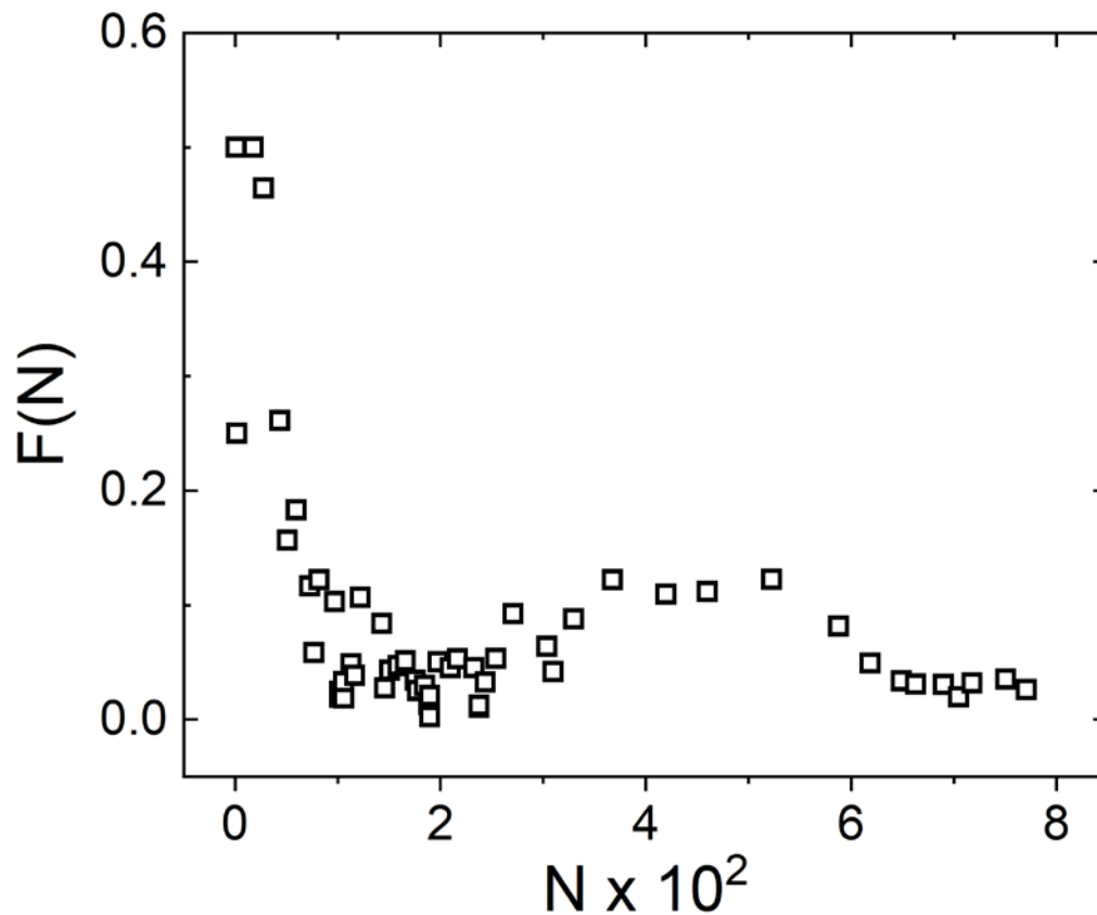
Fig. 3: Plots of F(N) = N^{-1} \frac{dF(N)}{dN} vs N for cumulative cases in Sri Lanka.
