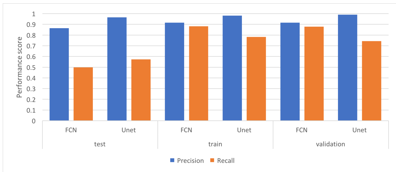
Fig. 6 Performance results, in terms of precision and recall scores, for the segmentation approaches in train, validation and test data sets.
