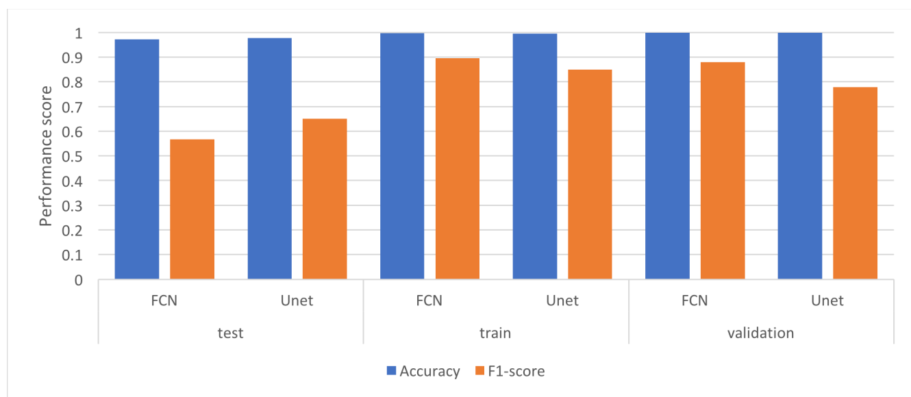
Fig. 5 Performance results, in terms of accuracy and F1 scores, for the segmentation approaches in train, validation and test data set.
