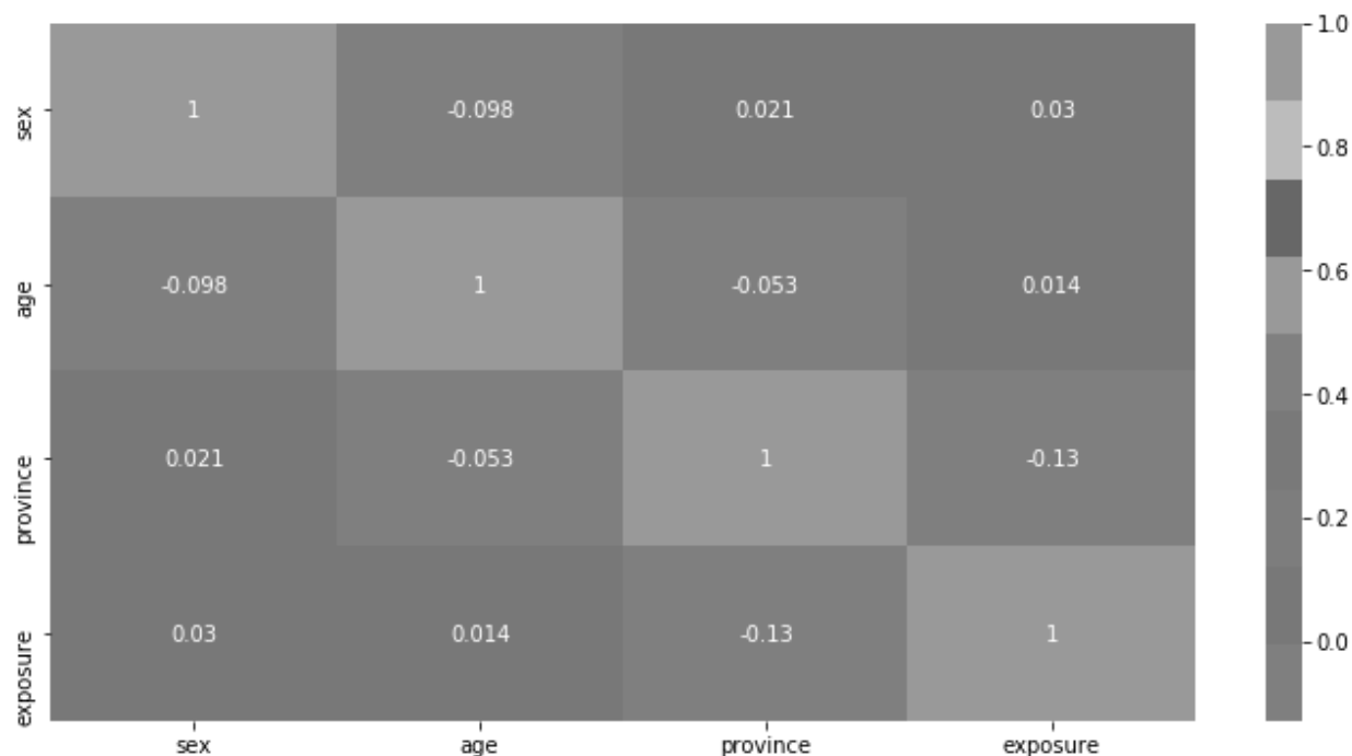
Figure 2. Correlation among predictors
