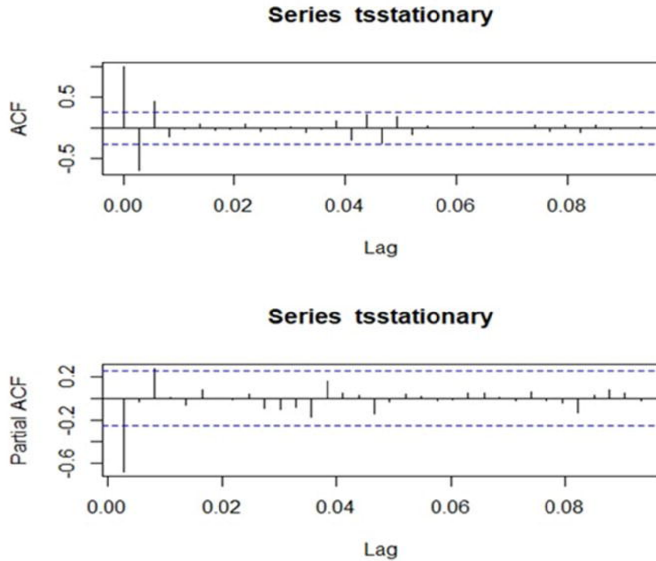
Figure 4 ACF and PACF plots to determine the candidate models
