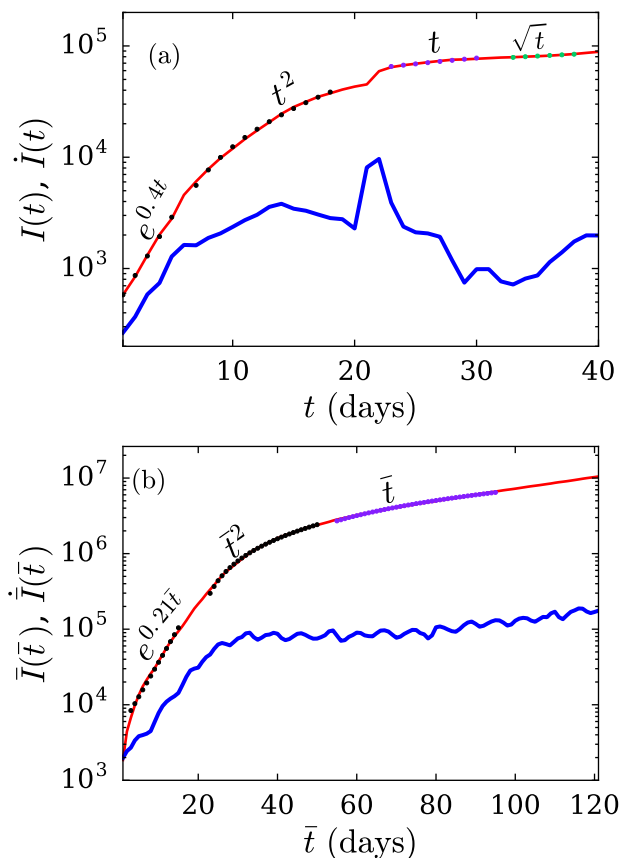
Figure 2: (color online) For the COVID-19 epidemic, the semi-log plots of total infected individuals ( I(t) ) vs. time ( t ) (red curves) for (a) Part 1: from January 22 to March 01 (comprising mostly of China), (b) Part 2: from March 02 to June 30 (world other than China). In Part 2, \bar{t} = t - 40 and \bar{I}(\bar{t}) = I(t) - I(t_0) = I(t) - 88000 . The blue curves in the plot describe the derivatives of I(t) . The dotted curves represent the best-fit curves listed in Table 2.
