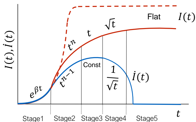
Figure 8: (color online) A schematic plot for time evolution of COVID-19 pandemic in a generic country. The red dashed curve is the path followed by the cumulative infections ( I(t) ) without any intervention (lockdown, contact tracing etc.). The solid red curve is the plot for I(t) with interventions, while the blue curve represents the daily infection cases ( \dot{I}(t) ). The five stages of the evolution are shown as Stages 1 to 5. The I(t) curve transitions from convex to concave nature during stage 3. Stage 5 corresponds to the flattened region.
