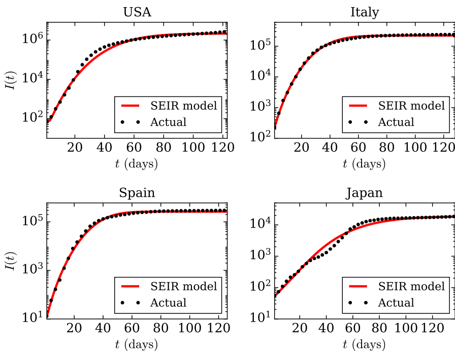
Figure 4: (color online) For the COVID-19 pandemic, semi-log plots of total infected individuals ( I(t) ) vs. time ( t ) (black dotted curves) for USA, Italy, Spain and Japan from the available data at worldOmeter [40] till June 30. The red curves are the best-fit curves using the SEIR model described in Sec. 4.
