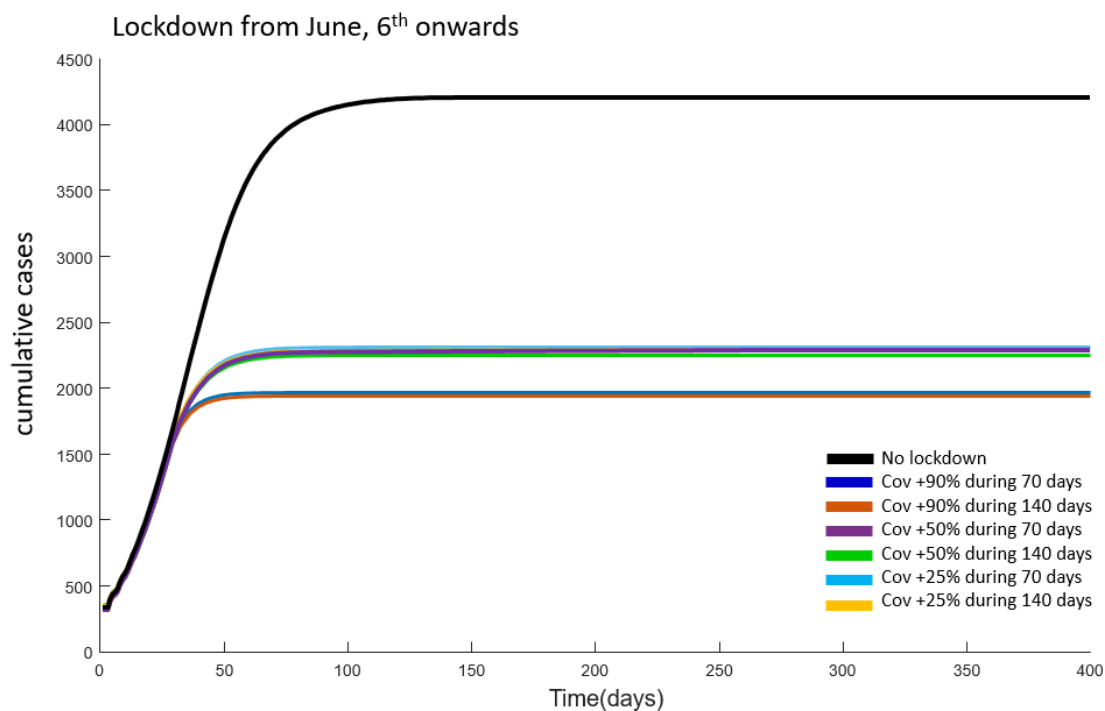
Figure 4. Effect of Lockdown Coverage(+%) and duration beginning at June 6 th at Rio de Janeiro State, with Re = 1.28 : cumulative cases. Initial conditions: 100 active and 240 immune/deceased (see text). 50 simulations. See color captions.
