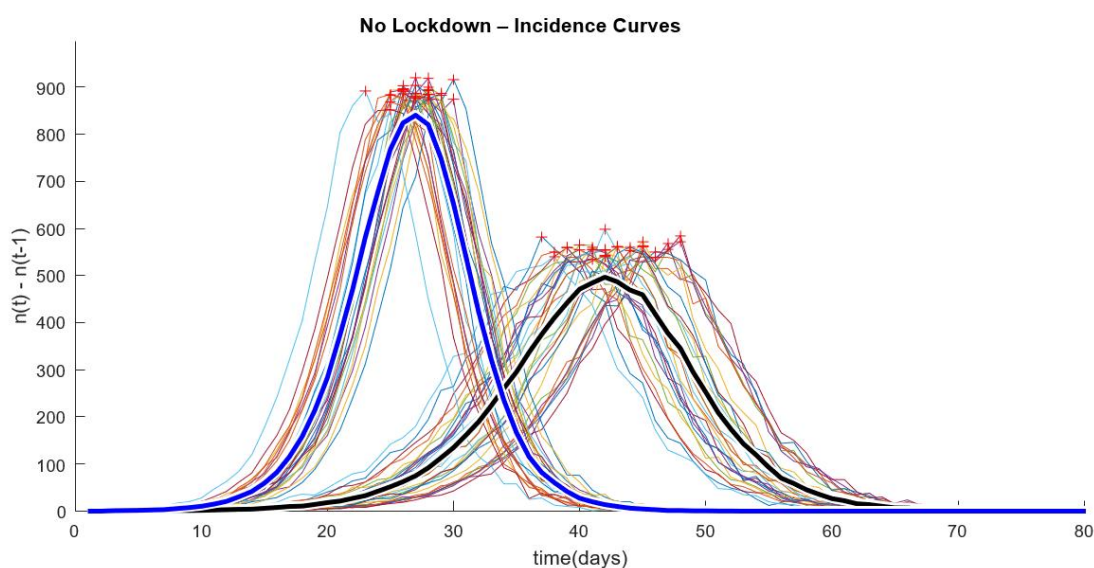
Figure 01. Incidence curves in a sample with thirty simulations for RO of 2.7 and 5.7. Mean values are plotted above the corresponding samples, in black and blue, respectively. Peaks are indicated with red crosses. See table 01.
