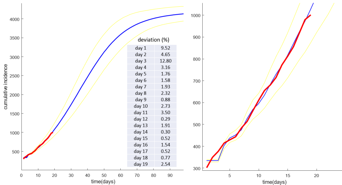
Figure 2. Evidence of validity – real data series upon modeled data from May 6 th to 25 th for State of Rio de Janeiro. Red: normalized data about cumulative mortality (see text). Blue: predicted data about epidemic progression (cumulative cases, mean of 50 simulations). Yellow: ± 2 standard deviation of mean. Table: variation rate (%) between real (normalized) and predicted data.
