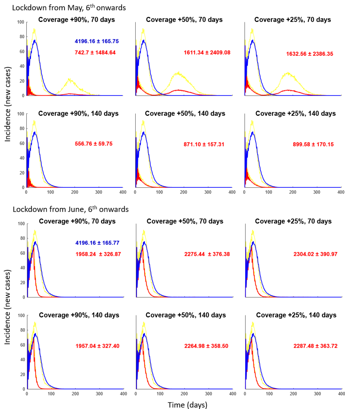
Figure 3. Effect of Lockdown Coverage(+) and duration with Re = 1.28 (Rio de Janeiro scenario).
