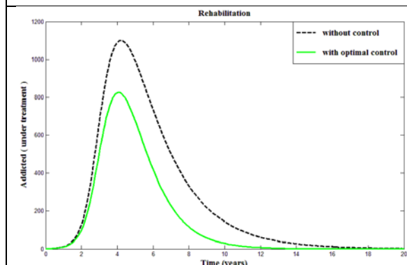
Figure 5.8. Dynamics of addicted population in rehabilitation using family based care ( u_2 ) as optimal control
