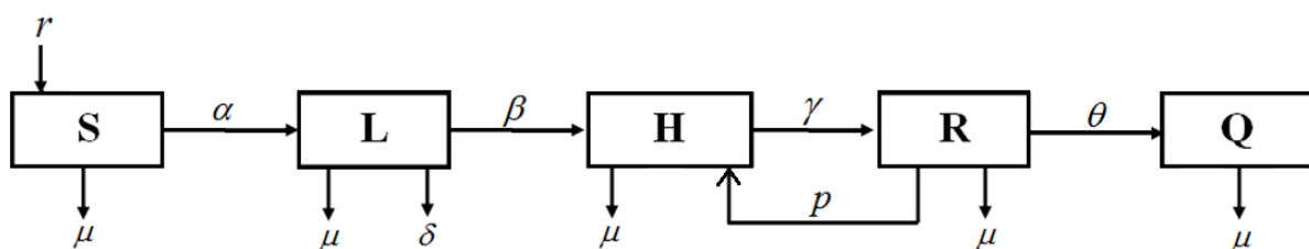
Figure 2.1. Compartmental representation of drug addiction model
