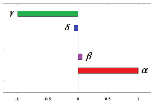
Figure 5.1. Effects of parameter variations on R_0
