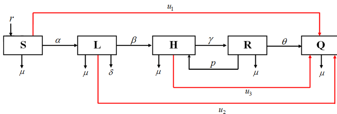
Figure 3.1. Compartmental representation of drug addiction model with control
