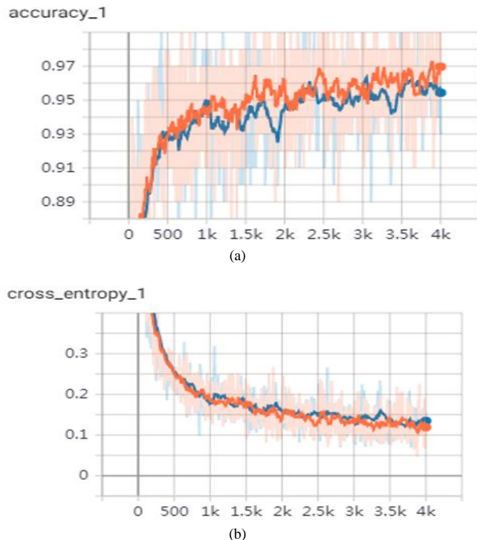
Fig. 9. (a) Training and validation accuracy of model and (b) cross entropy. Orange curve indicates the training cross-entropy/accuracy and blue curve indicates the validation cross-entropy/accuracy.
