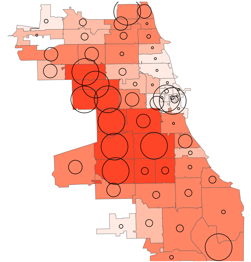
Cumulative Incidence
