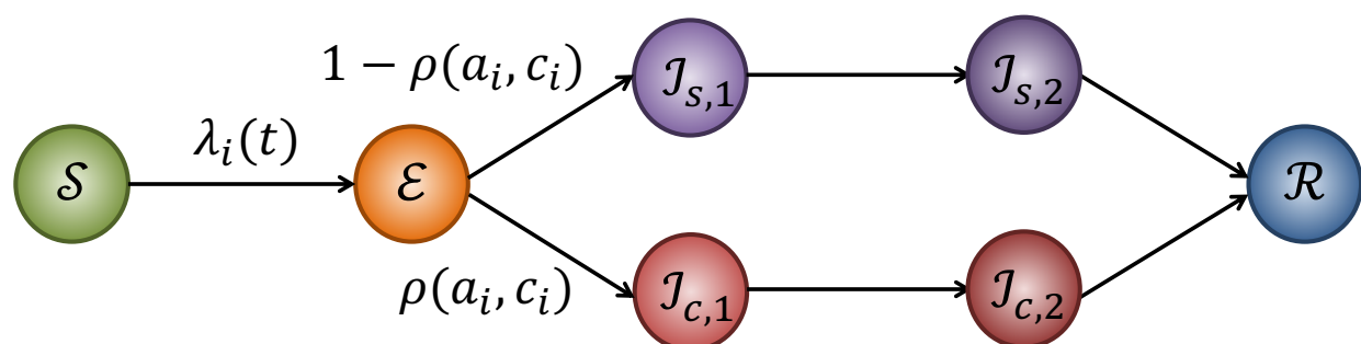
Figure A1. Structure of stochastic individual-level model of COVID-19 transmission. The labels of each state correspond with definitions in Table A1. The prob(a,c) refers to the probability of being a clinical or sub-clinical with force of infection lambda.
