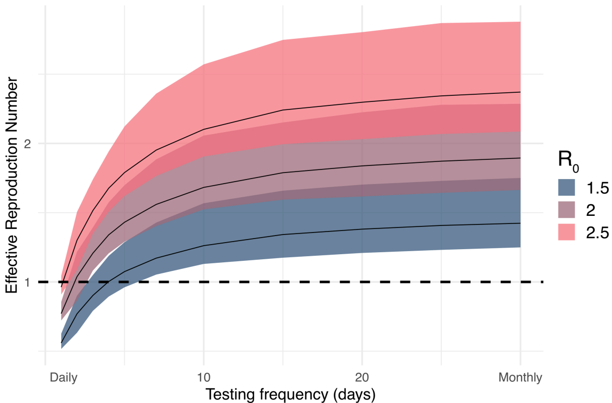
Figure 2: Projected effective reproduction number in a susceptible workplace under different testing scenarios. We estimated the effectiveness of increasing frequency of routine PCR testing to reduce the effective reproductive number, under various assumption on the true underlying basic reproductive number. The x-axis refers to the frequency of PCR testing simulation from daily (testing frequency of 1 day) to once a month (testing frequency of 30 days). The y-axis represents the effective reproductive number ( R_e ), which is the average number of people infected by the average person with SARS-CoV-2. The goal is to reduce the effective reproductive number below one to prevent ongoing transmission. Bounds represent the interquartile range.
