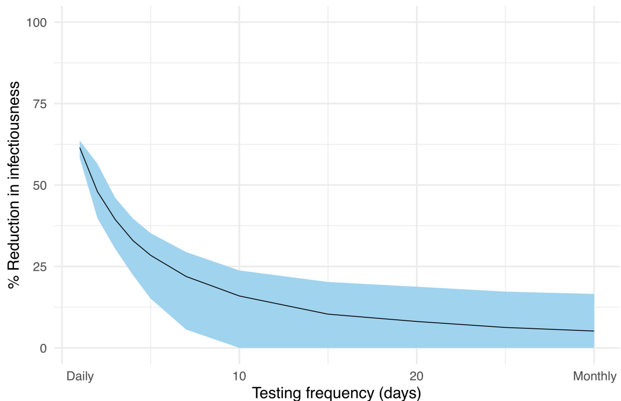
Figure 1: Projected effectiveness of routine PCR testing frequency on reduction on transmission for high risk workers. The x-axis refers to the frequency of PCR testing simulation from daily (testing frequency of 1 day) to once a month (testing frequency of 30 days). The y-axis represents the reduction in total number of infectious days attributable to each testing strategy. We estimate 40% of cases to be sub-clinical. Error bars represent the interquartile range of projected reduction, varying sensitivity and specificity of the PCR test and assumptions on natural history of transmission.
