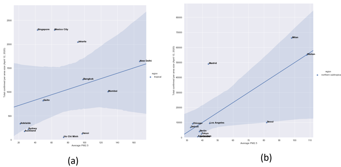
Figure 10: Regression analysis between confirmed cases and average of PM2.5 in (a) tropical and southern subtropical cities and (b) northern subtropical cities.
