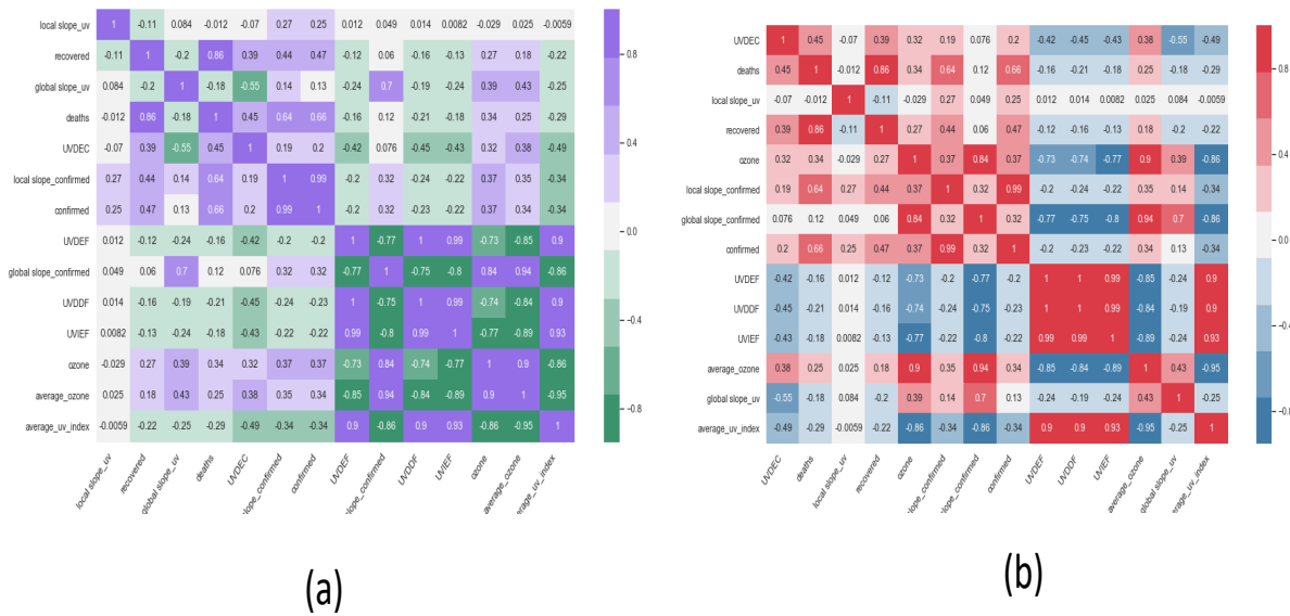
Figure 8: (a) Correlation map between parameters of the world. (b). Correlation map between parameters of China.
