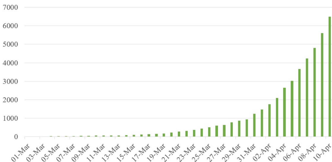
Figure 2: Day-wise active COVID-19 cases in India
