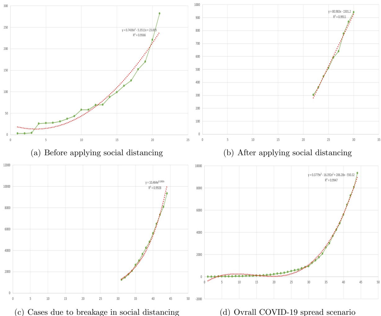
Figure 3: Active COVID-19 cases spread scenarios in India
