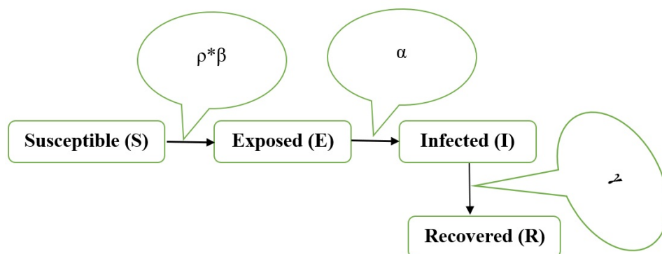
Figure 1: Proposed Mathematical Model With Social Distancing
