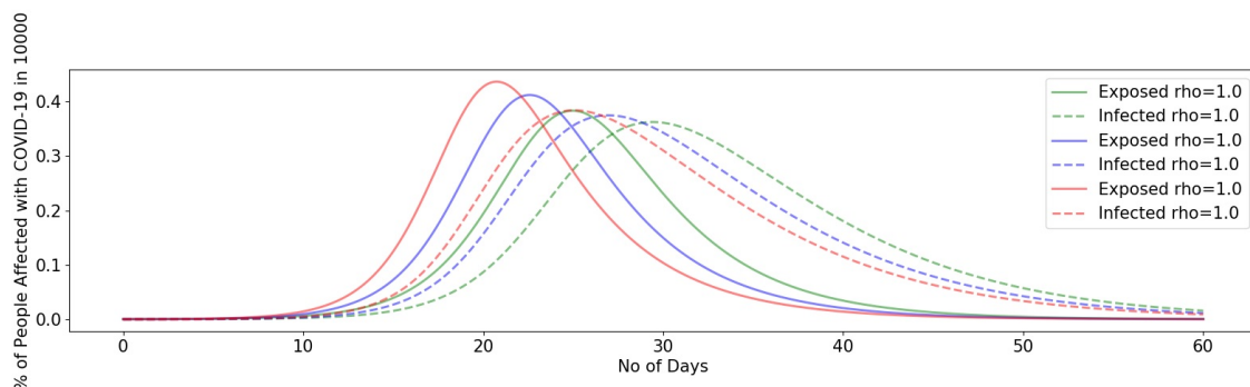
Figure 4: COVID-19 Spread before applying social distancing with \rho = 1
