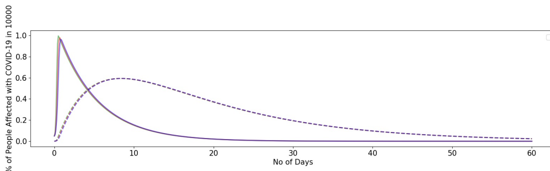
Figure 6: COVID-19 Spread due to breakage in social distancing
