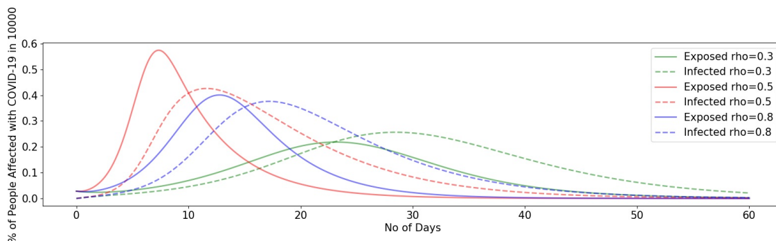
Figure 5: COVID-19 Spread after applying different social distancing rates
