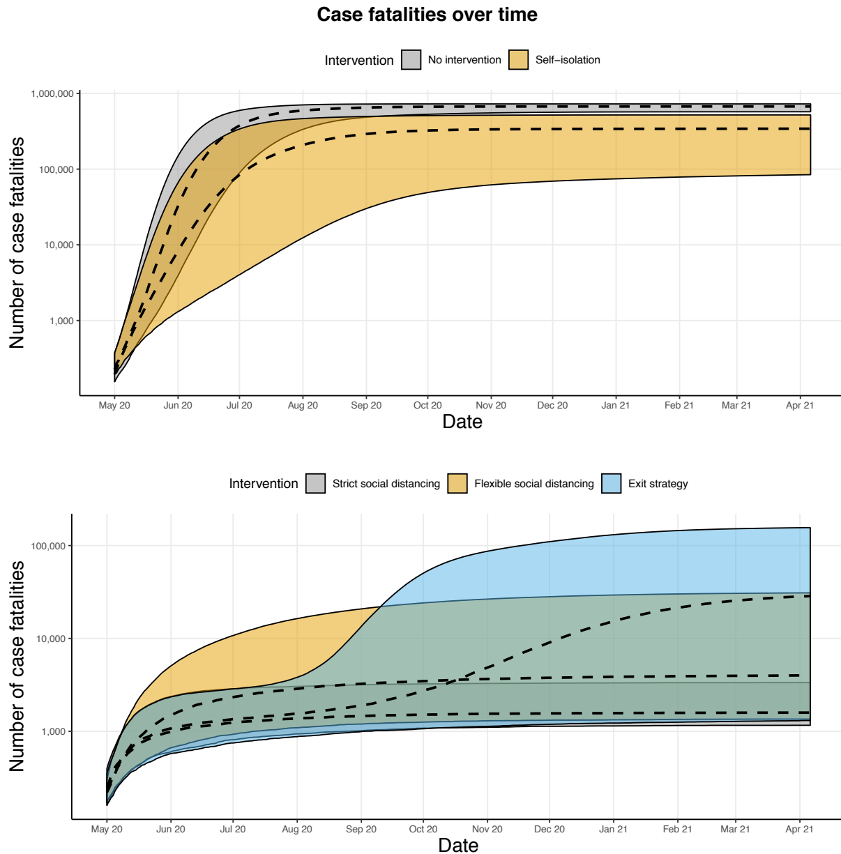
Figure 3: National-level estimates of cumulative case fatalities spread with sensitivity bands of infectivity of asymptomatic patients
