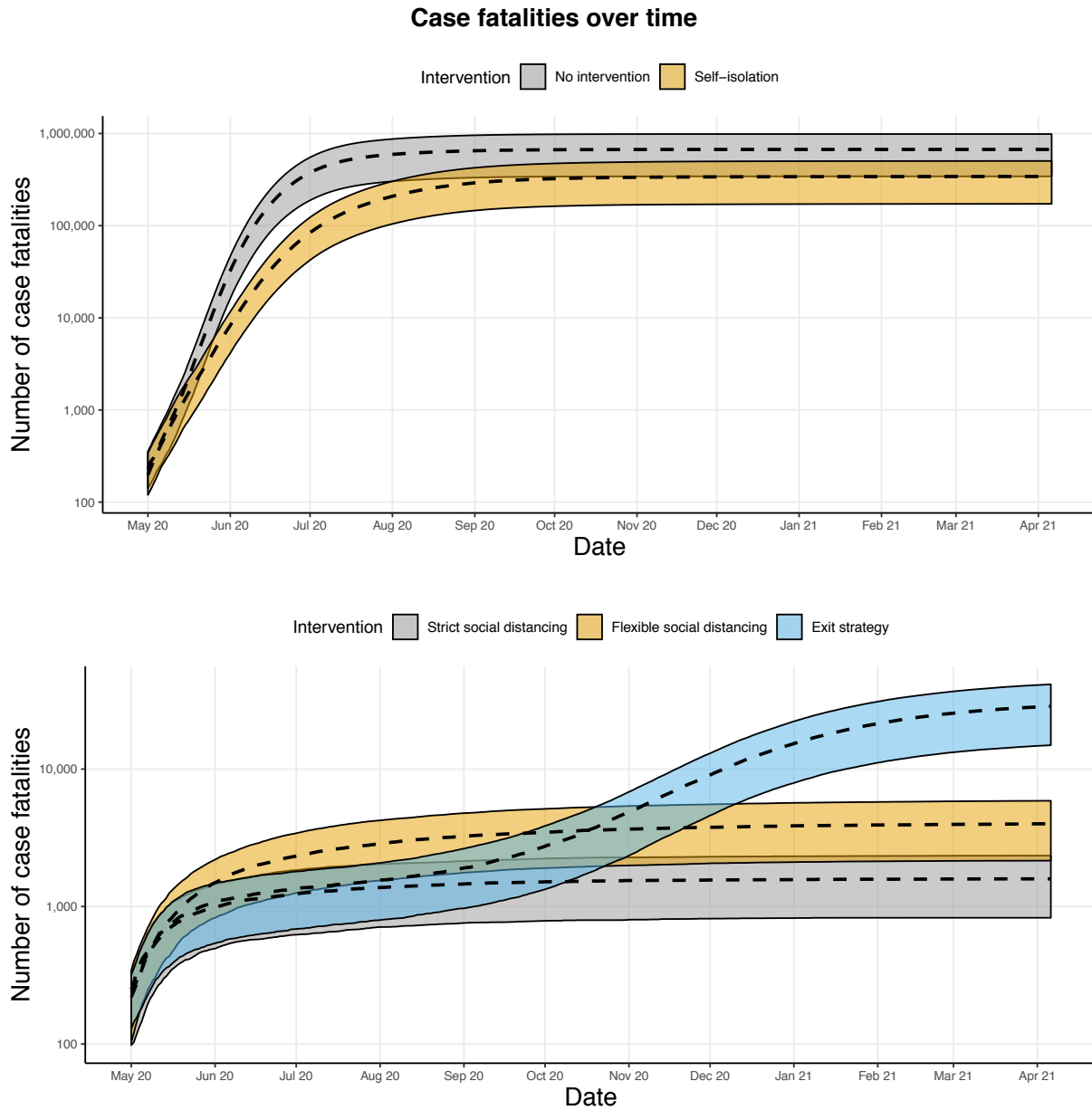
Figure 2: National-level estimates of cumulative case fatalities spread with sensitivity bands of fatality rates
