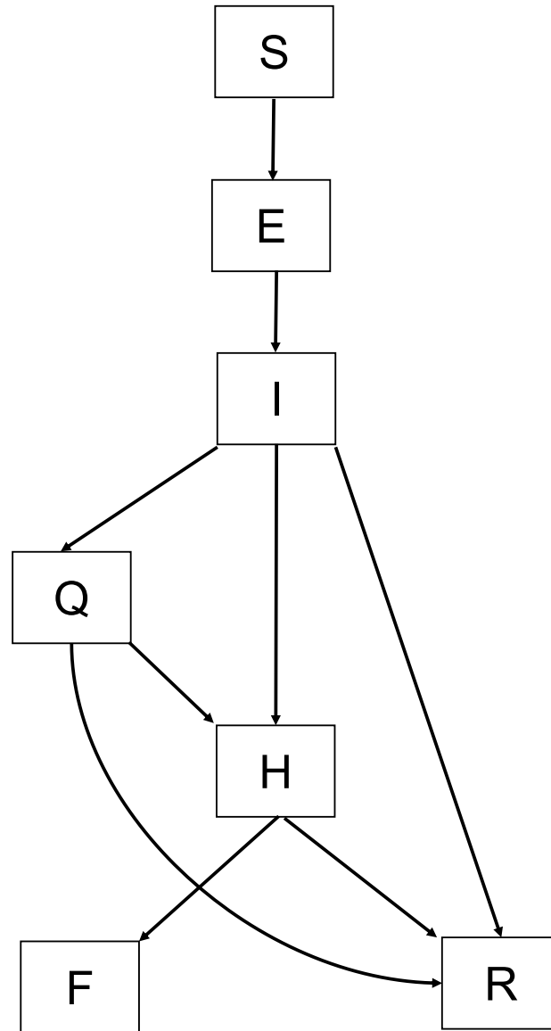
Figure 1: Transition diagram of this compartment model
