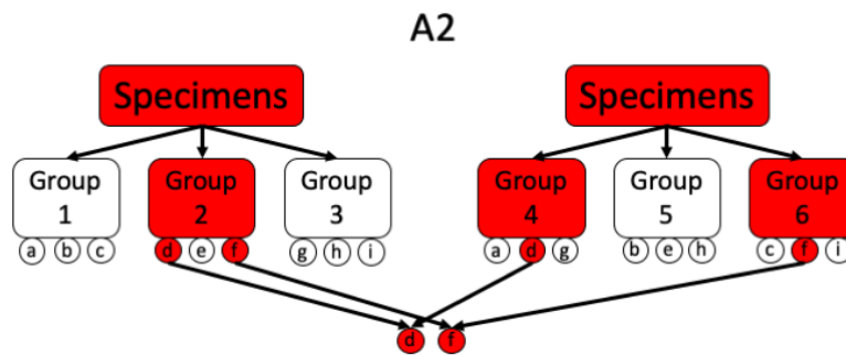
Figure 4: Illustration of a simple A2 procedure where the positive individuals are uniquely determinable after the first stage. Every individual a, b, c, \dots, i gets pooled exactly twice.
