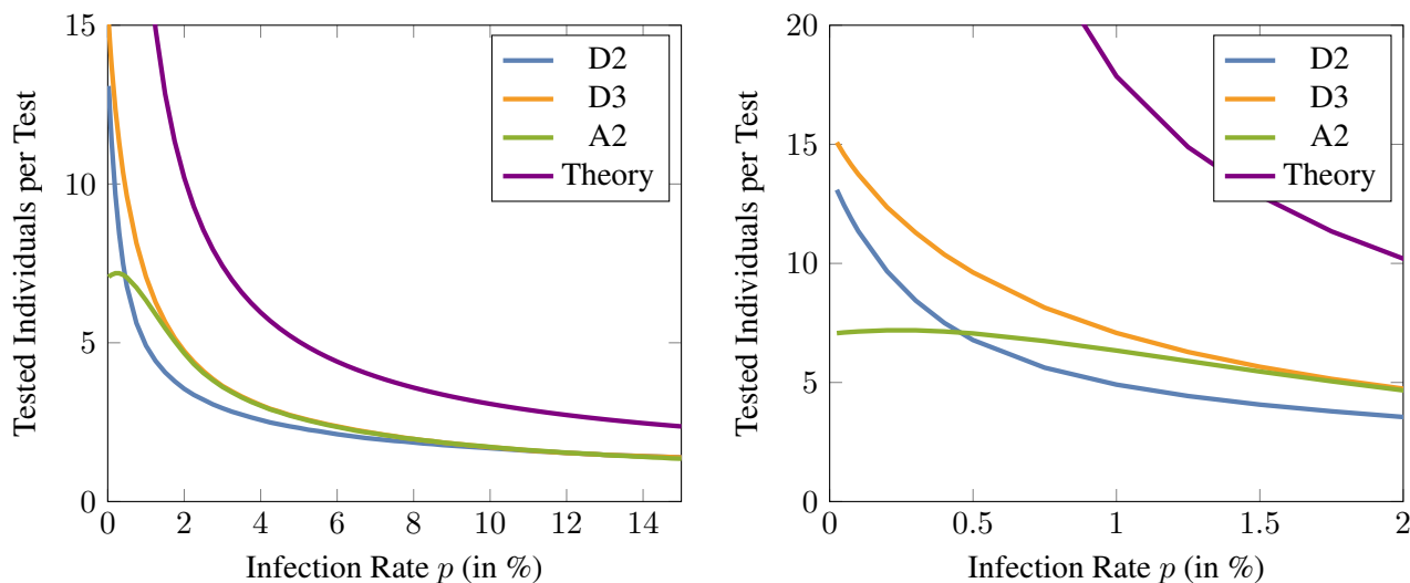
Figure 6: Number of individuals that can be tested per test available for the different adaptive methods. Here, the sensitivity and specificity are assumed to be 99%. The theoretical bound given by [45] is also shown for a comparison and the maximum group size is assumed to be 16. The figure on the right is a zoomed version of the left figure and illustrates the low prevalence regime of infection rates up to 2%.
