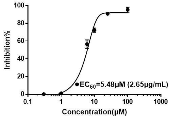
Baloxavir
