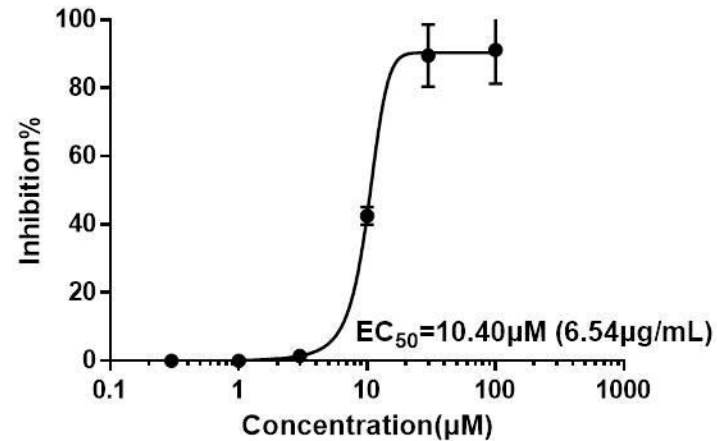
Lopinavir
