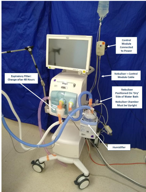
Figure 1. Ventilator circuit and nebuliser set-up
