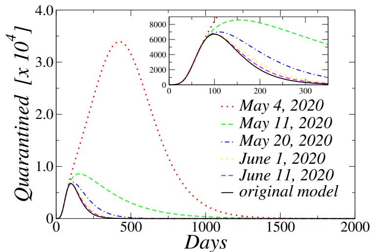
FIG. 5. (Color online) Time evolution of the number of Quarantined (Q) individuals. The full line represents the main result of section II.B, i.e., the original model with isolation policies ( k_0 = 0.033 ). The other curves represent the relaxation of such policies, starting from the days t' indicated in the graph. The inset shows a zoom of the smallest peaks. One can see that after June 1, 2020 there is no considerably change in the peak.
