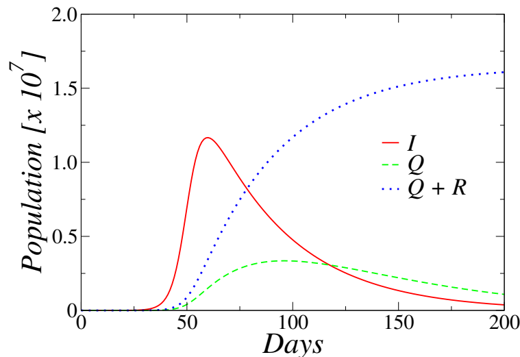
FIG. 2. (Color online) Time evolution of the number of Infected ( I ), Quarantined ( Q ) and total confirmed cases ( Q+R ) predicted by the SIQR model, obtained by the numerical integration of Eqs. (1) to (4). The parameters are I_0 = 13 , \beta = 0.3036 , \eta = \alpha = 0.0127 and \gamma = 0.02 .
