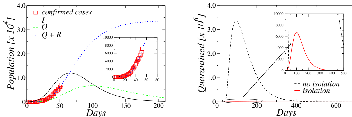
FIG. 4. (Color online) Left panel : Time evolution of the number of Infected ( I ), Quarantined ( Q ) and total confirmed cases ( Q+R ) considering all the data and isolation policies, obtained by the numerical integration of Eqs. (8) to (11). Data of confirmed cases are exhibited as well (squares). In the inset we show a zoom in the region of the current data (from March 5, 2020 through April 26, 2020), to highlight the agreement of the model with the data. Right panel : Flattening the curve: comparison between the predicted number of Quarantined individuals for the model with (full line) and without (dashed line) the implementation of isolation policies. The peak of the curve is considerably reduced. In both figures the parameters are I_0 = 24 , \beta = 0.32 , \eta = \alpha = 0.018 , k_0 = 0.033 and \gamma = 0.02 .
