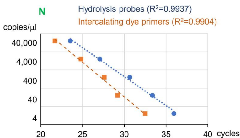
Figure 2. Standard calibration curve of hydrolysis probes and intercalating dye primers. The amplification of the N gene was compared using the N1 hydrolysis probe (blue) and the N set of primers for intercalating gene (orange) assay using dilutions corresponding to 4-40,000 copies of N gene per PCR reaction. The determination coefficient ( R^2 ) for the linear adjustment is indicated.
