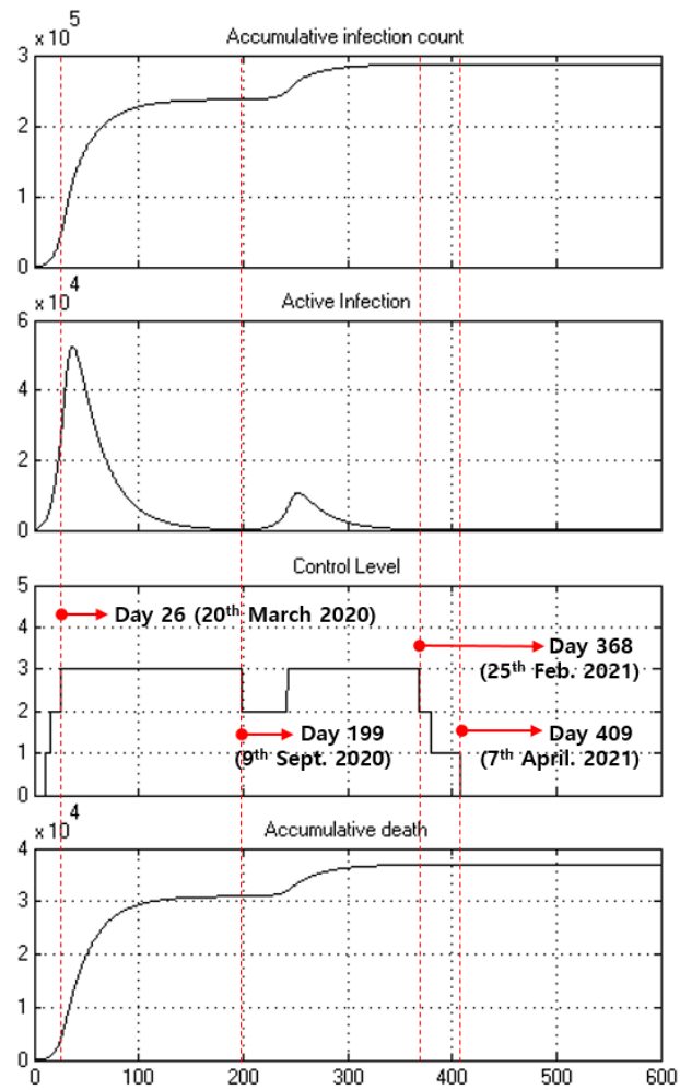
(b) Simulation of COVID-19 with the vaccine arrival on day 365
