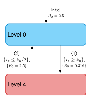
(a) A two-level control system captured as an HIOA (NZ-C3)
