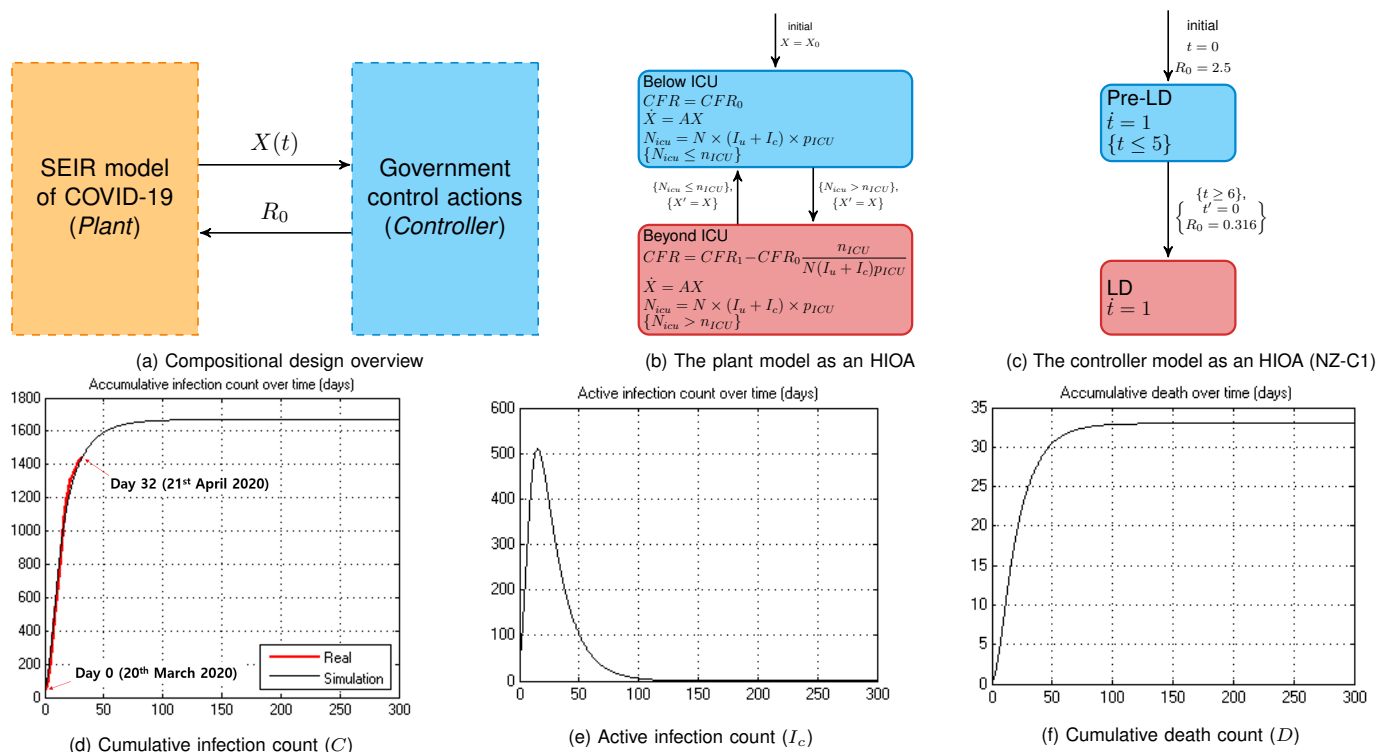
Fig. 1: The proposed compositional design of Compositional Cyber-Physical Epidemiology and simulation results. For (d), (e), and (f), day 0 corresponds to 20th March 2020. The first 32 days of (d) are compared with the available New Zealand data.
