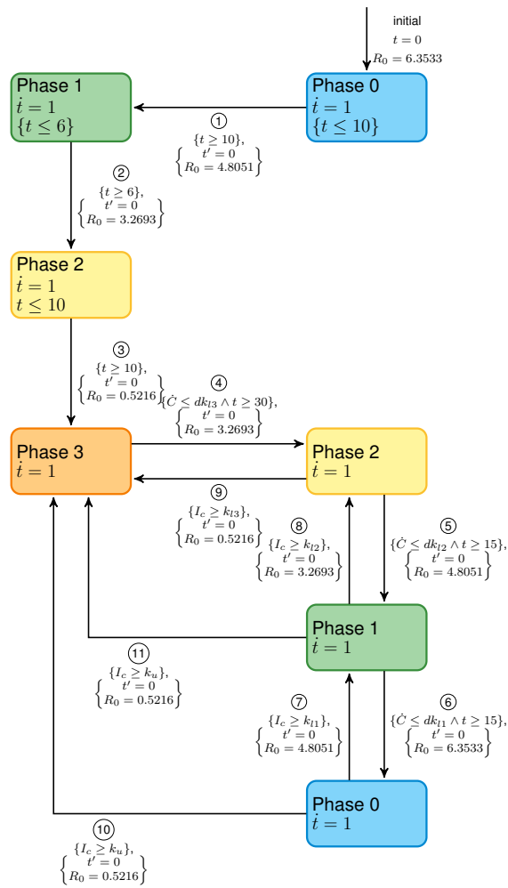
(a) A three-level control system captured as an HIOA (I-C1)
