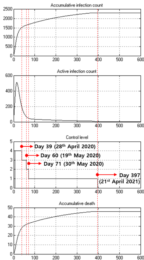
(b) Simulation of COVID-19 spread with vaccine arrival on day 365
