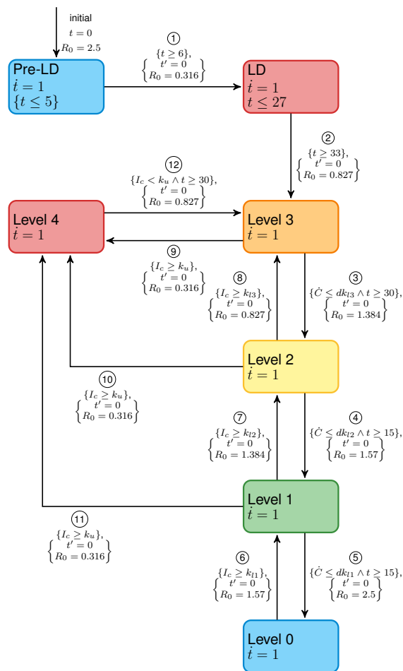
(a) The four-level alert system captured as an HIOA (NZ-C2)
