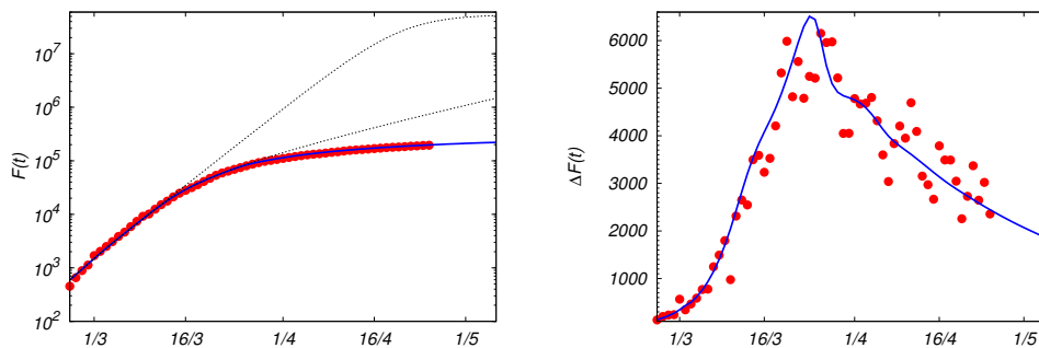
FIG. 3: (Left) Total number of infected persons over time, F(t) (red points), from official data for Covid-19 in Italy [5], where p = 6 \cdot 10^7 , up to 14th April. The blue line is the theoretical prediction F(t) as solution of Eq. (16), with initial conditions, fixed at t = 0 the 21th February, F_0 \simeq 150 , and r = r_1 \simeq 0.23 ( \mathcal{R}_0 \simeq 2.65 ), and using the profile for the infection rate given by Eq. (17), with the parameters reported in Fig. 2. The gray dotted lines are the expected curves for F(t) if the first and the second containment measures (8-11th March and 22th March) had not been taken. (Right) Daily number of infected persons, \Delta F(t) , compared with the theoretical \frac{dF(t)}{dt} from the solution of Eq. (16).
