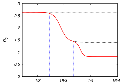
FIG. 2: Basic reproduction number \mathcal{R}_0 = r(t)\delta t , as a function of time, based on the profile for the infection rate described by Eq. (17). We take \delta t about 11 or 12 days [4], t_1 between 13th and 14th March 2020, t_2 on 26th March, \tau_1 \sim 2 days, \tau_2 \sim 1 day. The starting value is \mathcal{R}_0 = r_1\delta t \simeq 2.65 and the intermediate value is \mathcal{R}_0 = r_2\delta t \simeq 1.45 , and a current value, \mathcal{R}_0 = r_3\delta t \simeq 0.85 . The vertical dotted blue lines point the dates of the main laws for the containment measures (8th-11th March and 22th March 2020). The gray dotted lines correspond to \mathcal{R}_0 in the absence of the first and the second containment measures.
