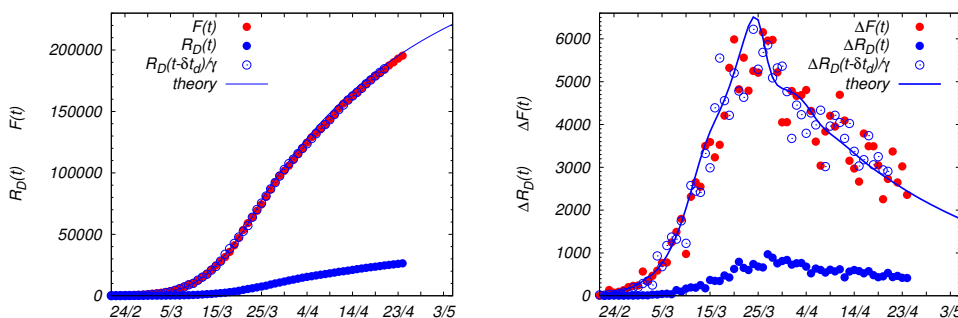
FIG. 4: (Left) Total number of confirmed cases of Covid-19 in Italy, F(t) (red dots), reported in Ref. [5], up to 25th April 2020, compared with the deceased cases, R_D(t) (blue dots), in the same period of time. If the numbers of died persons are shifted in time by \delta t_d \simeq 4 days and rescaled by \gamma^{-1} = 7 (blue circles) they perfectly overlap with the total numbers of cases. The blue solid line is theoretical prediction for F(t) , solution of Eq. (16). (Right) Daily number of infected persons, \Delta F(t) (red dots), and daily number of victims \Delta R_D(t) (blue dots). The blue circles are the daily number of victims after rescaling according to Eq. (19), with \delta t_d = 4 days and \gamma = 1/7 . The solid blue line is \frac{dF(t)}{dt} from the solution of Eq. (16).
