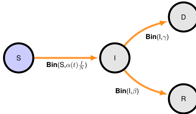
Figure 1: SIR-D as a time-varying Markov Chain. The notation \text{Bin}(n, p) corresponds the binomial distribution where n is the number of people in the prior state and p is the probability for an individual to move into the posterior state, e.g. p = \alpha(t) \frac{I}{N} is the probability for an individual in the susceptible population of size n = S to get infected.
