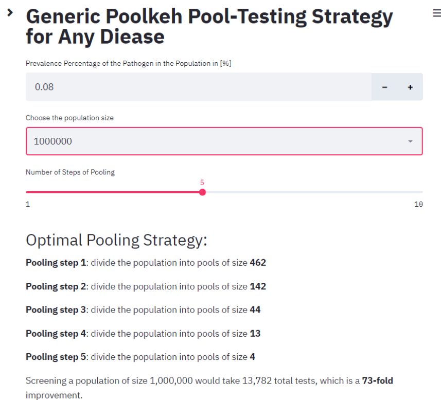
Figure 7: The Poolkeh Generic User-Interface.
