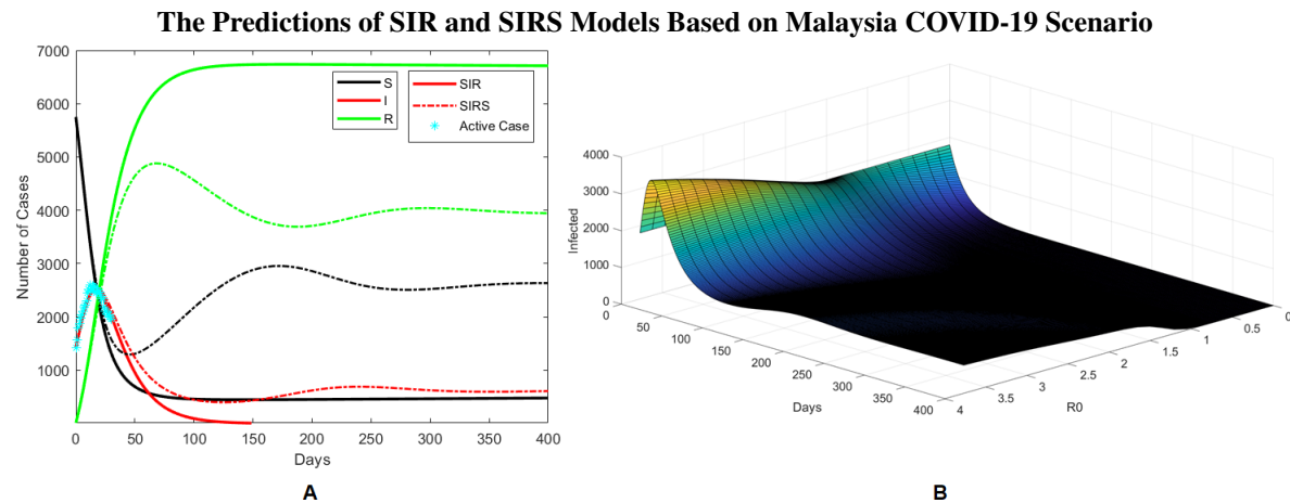
Fig. 1 Numerical simulation results of SIR ( \varepsilon = \alpha = 0 ) and SIRS ( \varepsilon > 0, \alpha = 0 ) models with the assumption of limited medical resources is relaxed. (A) Time series results of SIR (solid lines) and SIRS (dashed lines) models and comparison with the number of active cases in Malaysia (cyan asterick). (B) The daily number of active cases in Malaysia as R_{0u} varies based on predictions of SIRS model: as R_{0u} < 1 , the pandemic can be excluded; when R_{0u} > 1 , the pandemic persists for a long period of time. Other parameter values: \beta = 0.16 (fitted), \gamma = 0.058 (fitted), \mu = \nu = 0.00002^{14} , N = S + I + R and \varepsilon = 0.0009 (fitted).
