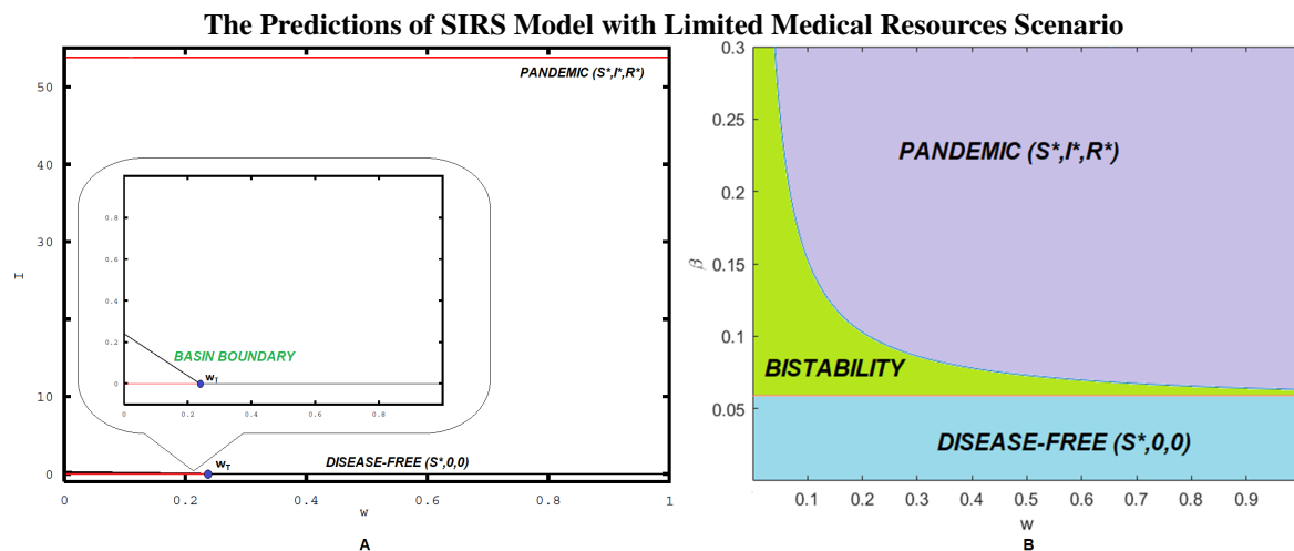
Fig. 2 Bifurcation analysis results of the model (1) with limited medical resources and possibility of false detection. (A) A one-parameter bifurcation diagram when \beta = 0.095 as \omega varies with threshold \omega_T represents transcritical bifurcation (blue point). (B) A two-parameter bifurcation diagram in (\omega, \beta) -plane with different colour regions represent transmission dynamics of the system. Other parameter values: \mu = \nu = 0.00002^{14} , N = S + I + R , \varepsilon = 0.0009 (fitted), \gamma = 0.053 (fitted) and \alpha = 0.01^9 .
