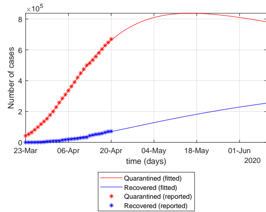
Fig. 2: Number of isolated cases predicted and recovered cases predicted by the model (15) for the United States.
