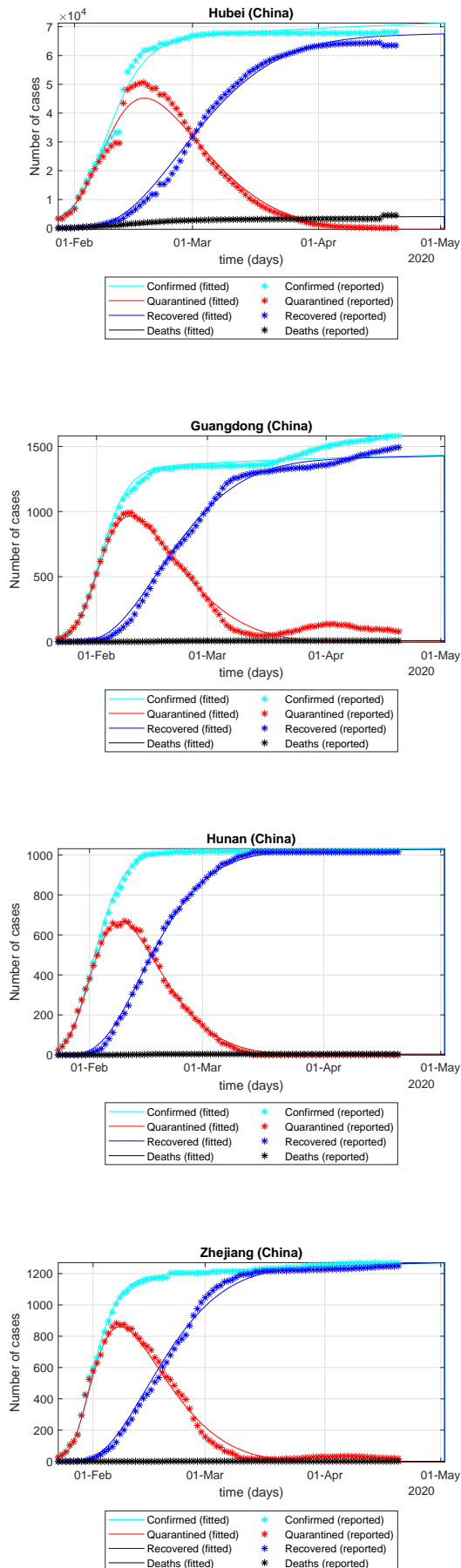
Fig. 3: The fitting effect of the improved model (17) on the outbreak in Hubei, Guangdong, Hunan and Zhejiang.
