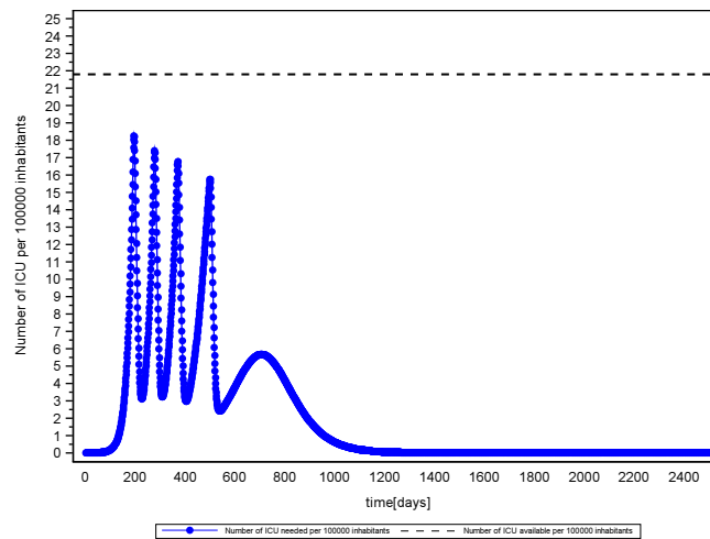
Fig 9. Mitigation and herd immunity strategy in a high performance health care system (Austria) and low rates of ICU admissions (2.2% of confirmed infected)
