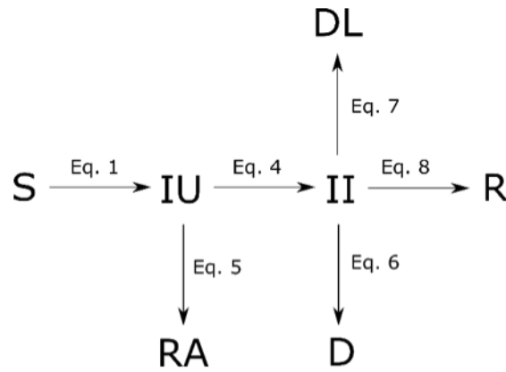
Fig 1. Schematic diagram of the adapted SIR model Schematic diagram of the adapted SIR model: susceptible (S), infected - infection unknown (IU), infected in isolation (II), resistant (R), resistant asymptomatic (RA), deaths (D), deaths caused by lack of ICU (DL), see also equations (Eq.) below
