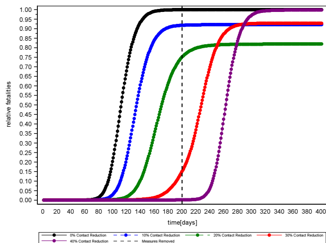
Fig 7. Relative fatality rates (1 = fatalities without intervention) in Scenario 2 with constant duration (200 days) and varying intensity of contact reduction
