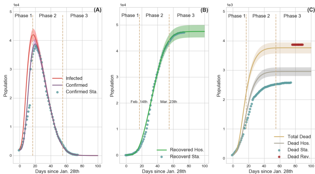
Figure 4: Comparison of the results generated by D-ICRD model and the time series data released by NHC. In this figure the dots denote official data and the lines denote the data calculated by D-ICRD in which the shadow areas denote the 95% confidence interval (CI). The entire pandemic in Wuhan is divided into three phases: Phase 1 [Jan. 23th - Feb. 14th]; Phase 2 [Feb.15 - Mar. 23th]; Phase 3 [Mar. 24th - ]. Sta. denotes the official statistical data and Hos. denotes the data counted in hospitals. (A) the curves of the existing infected and confirmed cases. The gap between the infected curve and the confirmed curve indicates the number of the infected but unconfirmed group (33). Most dots are located in the shadow areas except for Phase 1 because the health authorities clarified that there were many infected cases of underreporting. (B) The curve of recovered cases. The calculated data is slightly larger than the amounts counted in hospitals since the spontaneously curative patients are not included and a few medical institutions failed to connect with the information systems in time. (C) The curve of death cases. Blue dots denote the originally released data and the red dots denote the revised data by NHC. According to the revised data, mortality is seriously underestimated at Phase 1 and Phase 2, and the yellow curve is more representative of the death trend of COVID-19 pandemic.
