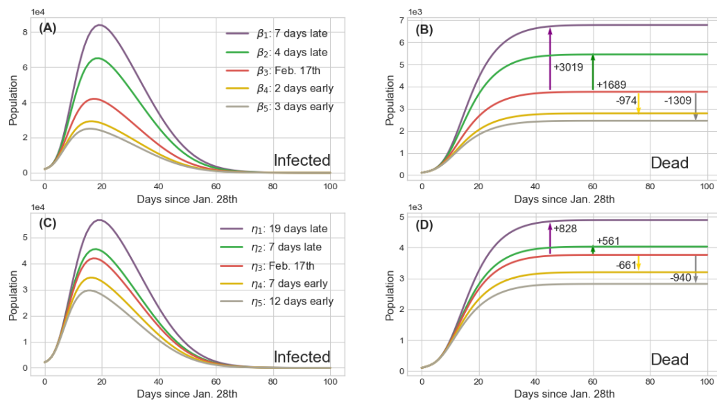
Figure 5: Impact of the implement time of isolation and investigation policies on transmission tendency of COVID-19 in Wuhan. The red lines are the results of the baseline policies selected in Fig. 2 and the other lines' colors are matched with Fig. 2 representing advance or delay the corresponding policy. The arrows show the increment or decrement of the death cases compared with the baseline of different policies. (A) and (C) The curves of infected persons calculated by the dynamical coefficient \alpha (isolation policy) and \eta (investigation policy) in Fig. 2 respectively. (B) and (D) The curves of deaths corresponding to (A) and (C) and they provide the statistic evidences how public health interventions save the lives of people.
