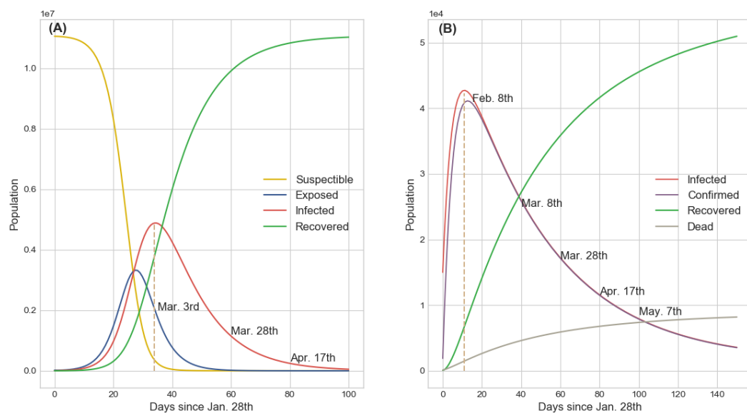
Figure 3: Results from the numerical simulations about COVID-19 transmission tendency of SEIR and S-ICRD models. (A) SEIR predicts that the existing infected cases would reach a peak of 4,885,672 on Mar. 3rd and the pandemic would be basically blocked on Apr. 17th in Wuhan. More than half of the population would be infected by COVID-19 but the fraction of exposed population is less than the infected population which is inconsistent with the observation. (B) S-ICRD predicts that the peak of the existing infected cases is 42,729 on Feb. 8th and the epidemic alert would be lifted after May. The forecasted number of infections is consistent with the actual data but the relative crucial time points and the final deaths have a great deviation with the observation in Wuhan since the constant coefficients are inappropriate to simulate the transmission dynamics of COVID-19.
