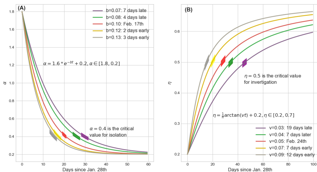
Figure 2: Mathematical representations of dynamical coefficients with respect to isolation policy and investigation policy respectively. (A) tuning the parameter b of \alpha can subtly regulate the implement time of isolation policy. We choose \alpha = 0.4 as the critical value for isolation which this policy is fully implemented. The practical isolation policy curve b = 0.10 (Feb. 17th) is selected as the baseline to compare results caused by advancing or postponing of this policy. The boundaries of \alpha \in [1.8, 0.2] are determined by the basic reproduction number R_0 and the duration from infected to infected. (B) tuning the parameter v of \eta can reflect the rate of community investigation for the infected but undiagnosed patients. We choose \eta = 0.5 as the threshold of daily investigation rate and v = 0.05 (Feb. 24th) as the baseline to compare the impact of the implement time of investigation policy to the pandemic trend. The boundaries of \eta \in [0.2, 0.7] are determined by the case capacity of the hospitals.
