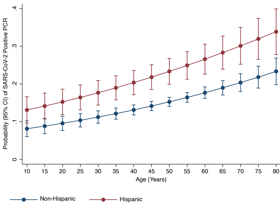
Figure 2a-b: Adjusted Probability and 95% Confidence Interval of Positive SARS-CoV-2 PCR in African American vs. Caucasian and Hispanic vs. Non-Hispanic by Age
