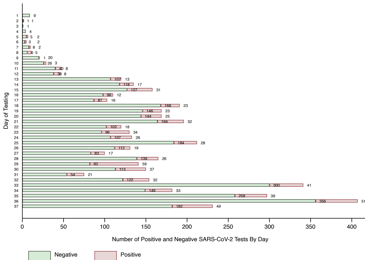
Figure 1: Schematic representation of the temporal sequence for total, positive and negative numbers of SARS-CoV-2 tests in the Houston Methodist CURATOR
