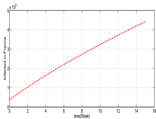
Figure 1.5: Model prediction for France
