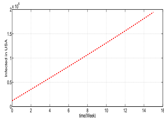
Figure 1.1: Model prediction for USA
