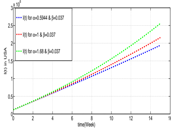
Figure 1.7: Model prediction for USA with different values of \alpha
