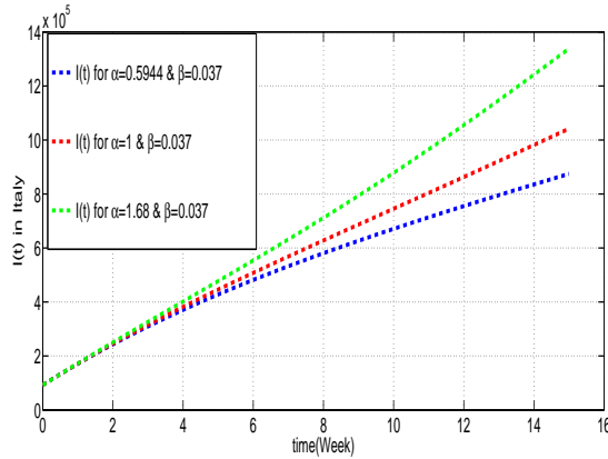
Figure 1.8: Model prediction for Italy with different values of \alpha
