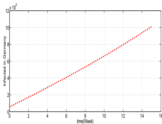
Figure 1.4: Model prediction for Germany
