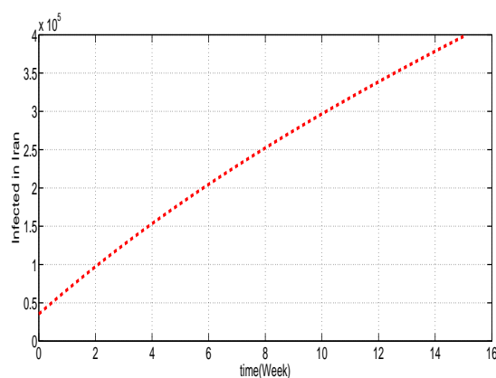
Figure 1.6: Model prediction for Iran
