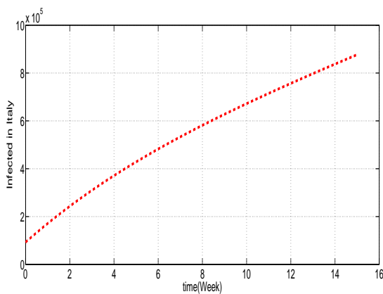
Figure 1.2: Model prediction for Italy
