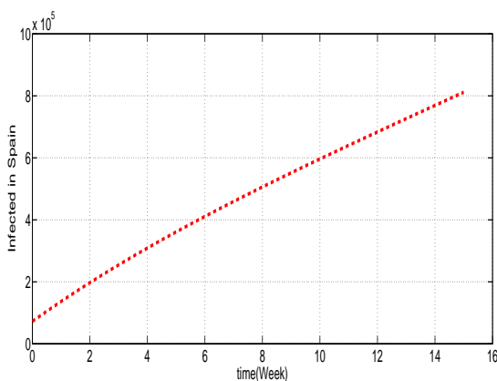
Figure 1.3: Model prediction for Spain
