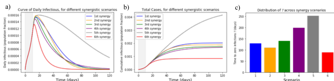
Fig. 7 Simulations of the 6 synergistic scenarios. (a) New cases curves, (b) Cumulative cases. The grey area indicates when measures are not yet in place. It is evident that scenarios leading to the same \hat{R} could show different patterns and suppression timing. (c) Distribution of times to zero infections T for different scenarios.
