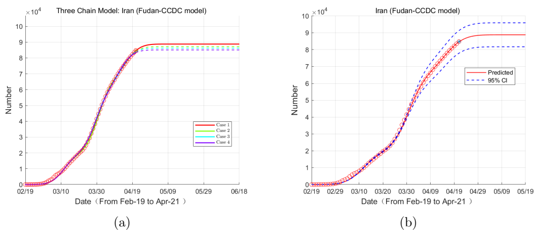
Figure 2: (a) Evolution of the number of cumulative confirmed cases based on the three-chain Fudan-CCDC model. Red circles: data; Red lines: model predictions; (b) Evolution of the number of cumulative confirmed cases based on the three-chain Fudan-CCDC model. Red circles: data; Red lines: model predictions; Blue dot line: 95% CI.
