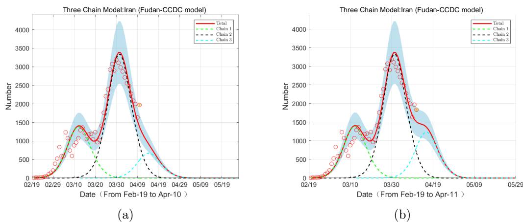
Figure 5: (a) Evolution of the number of increment confirmed cases based on the three-chain Fudan-CCDC model, with data from Feb 19 to Apr 10. Red circles: data; Red lines: model predictions; Green lines: first chain; Black lines: second chain; Blue lines: third chain. (b) Evolution of increment of confirmed cases based on the three-chain Fudan-CCDC model, with data from Feb 19 to Apr 11. Red circles: data; Red lines: model predictions; Green lines: first chain; Black lines: second chain; Blue lines: third chain.
