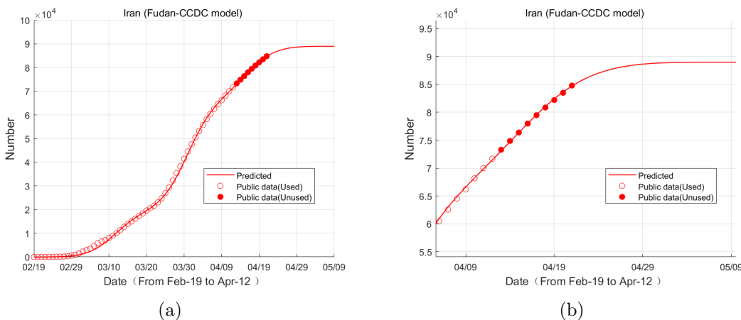
Figure 4: (a) Comparison of forecast results on April 12 and real data; (b) An enlarged version of (a).
