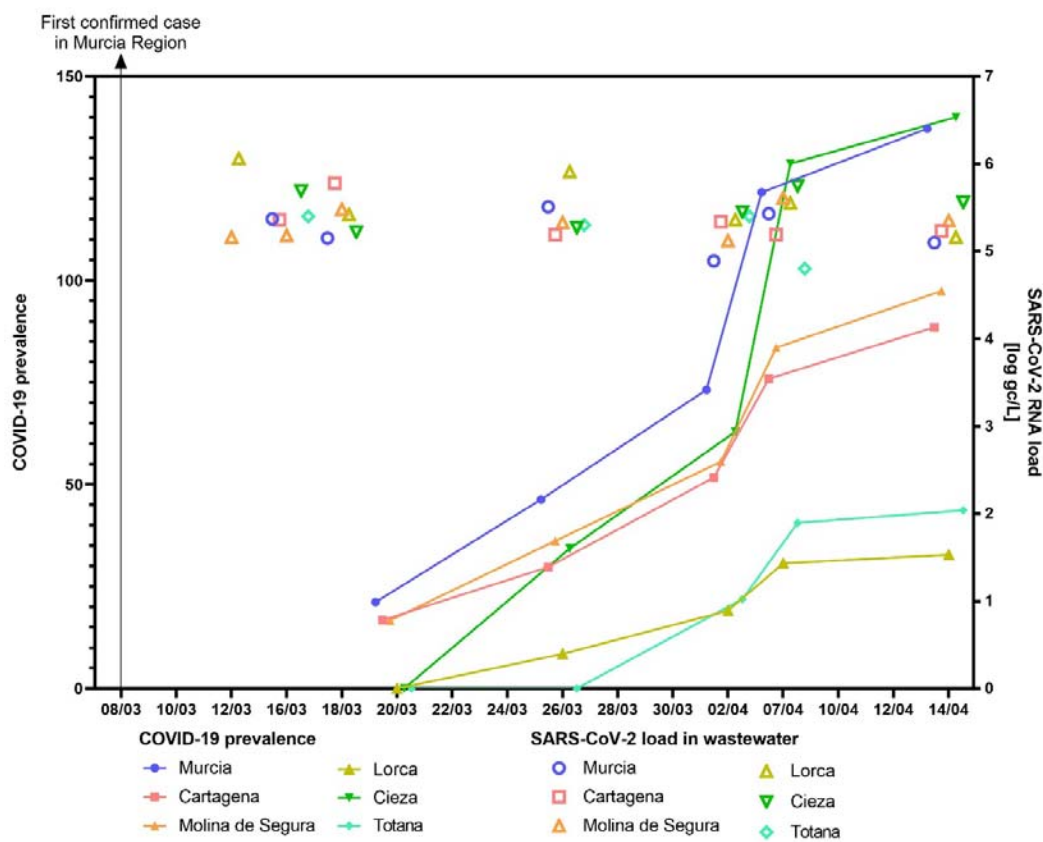
482 Figure 3. Epidemiological surveillance of COVID-19 by wastewater SARS-CoV-2 RT- 483 qPCR in six municipalities.
